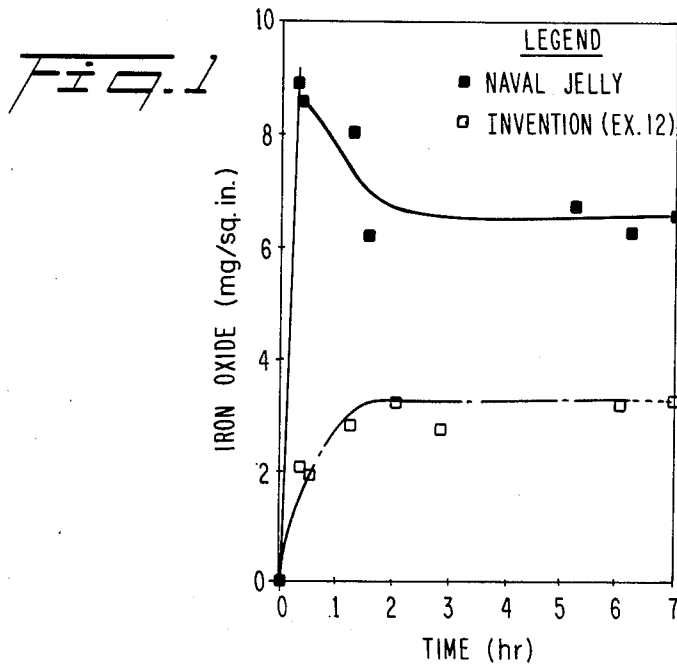
RUST REMOVAL vs. TIME FOR PRODUCT COATINGS
