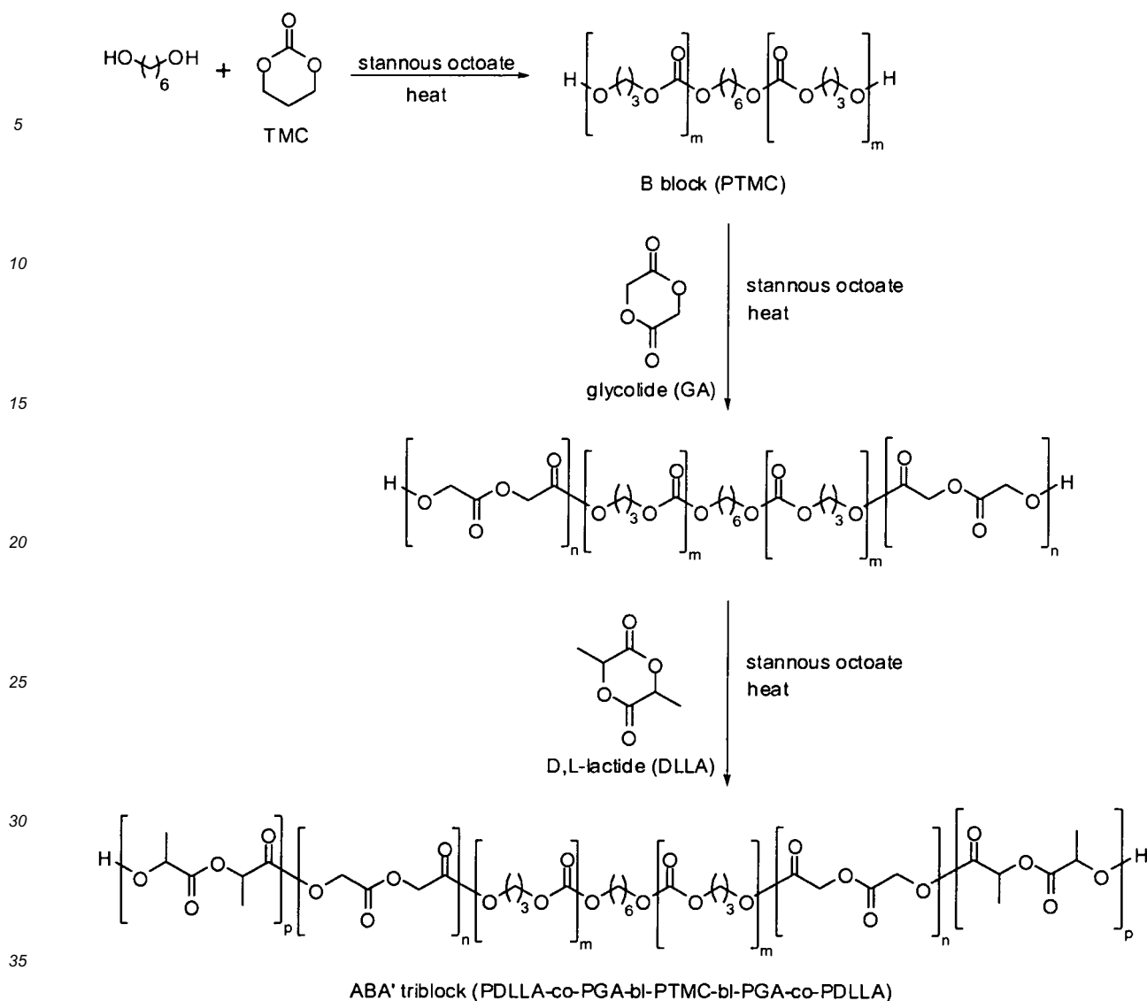
40 Scheme 1. Synthesis of poly(D,L-lactide-co-glycolide-bi-trimethylene carbonate-bi-glycolide-co-D,L-lactide) via ring-opening polymerization
