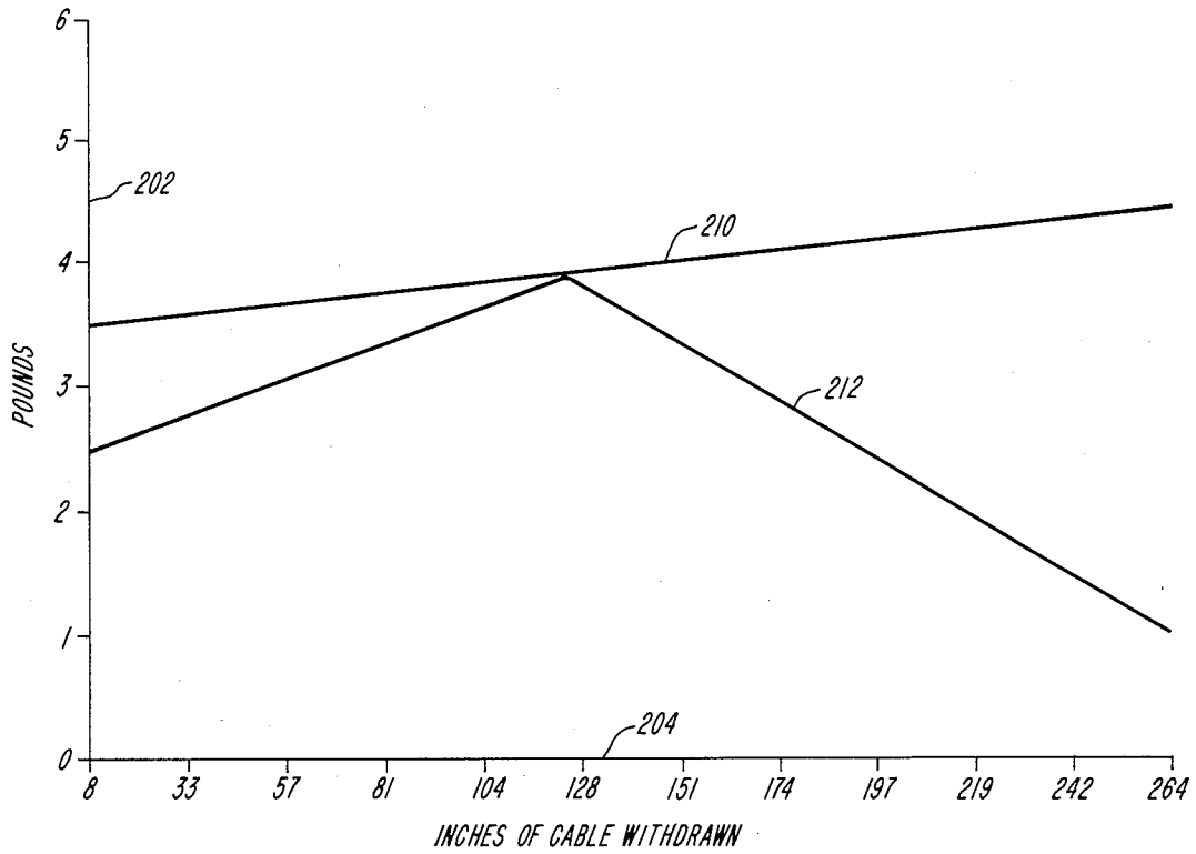
FIG. 8 (PRIOR ART)
