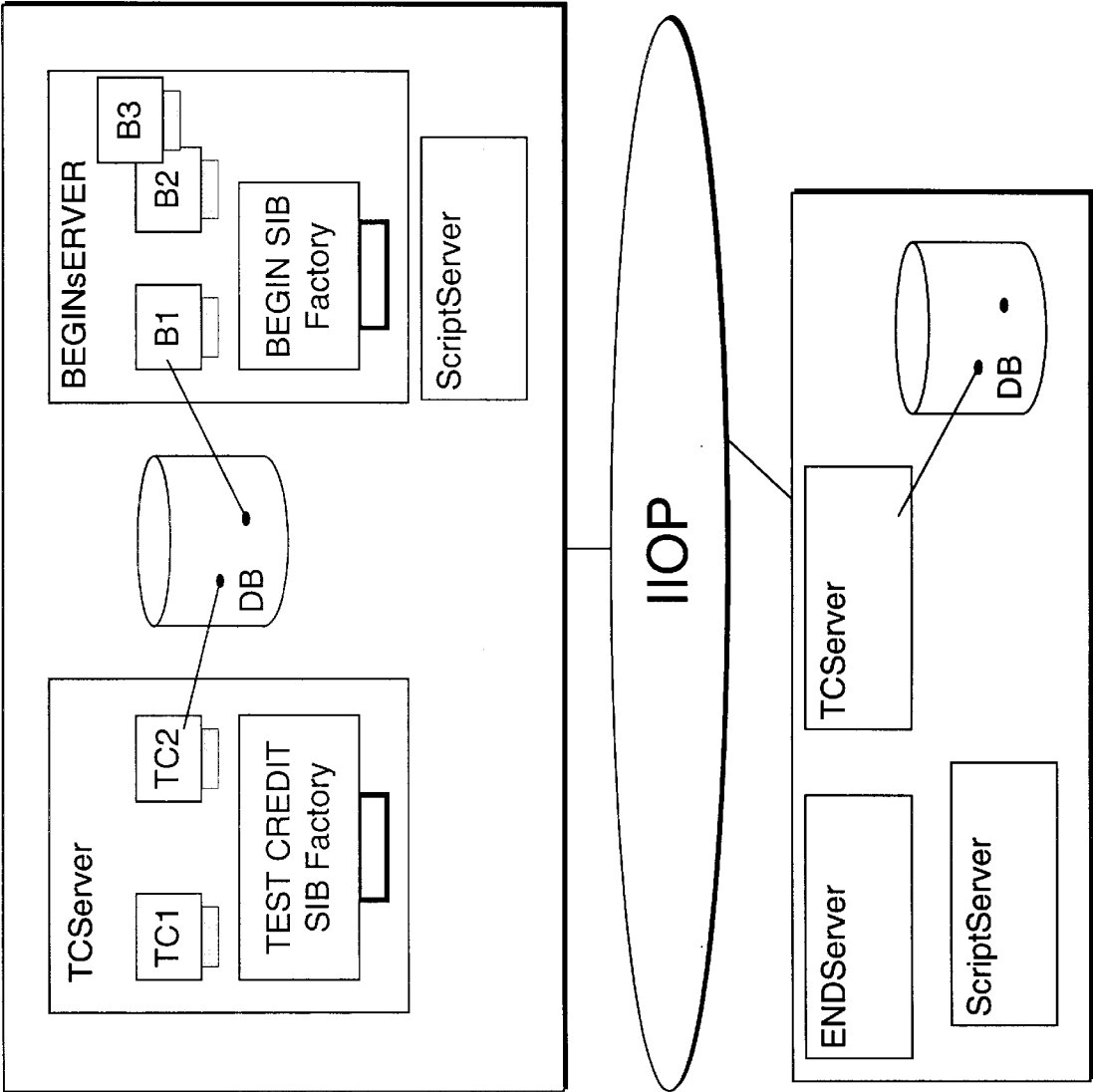
FIG. 3 Architecture 2
