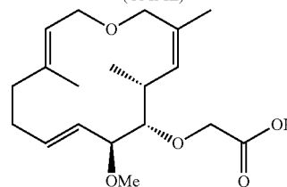
Carboxymethyl migraether (CMME)
