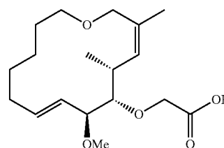
Carboxymethyl migraether (CMME)
