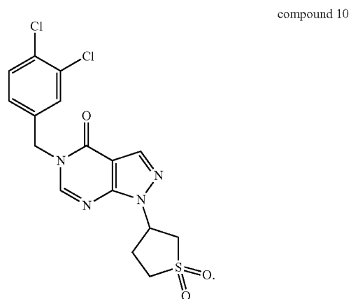
compound 10
