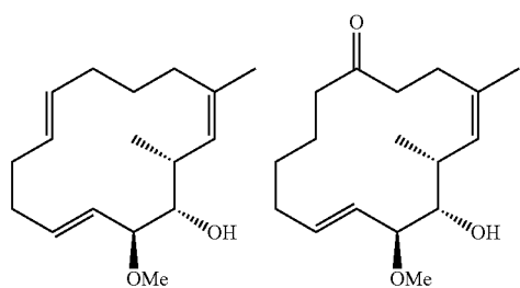
Dehydro migraether (DHME)
