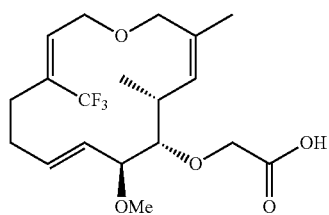
Carboxymethyl dehydromigraether (CMDME)
