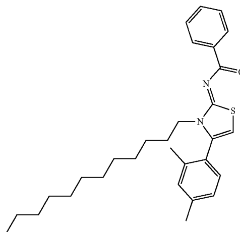
compound 6
