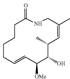
Dehydro migraether (DHME)
