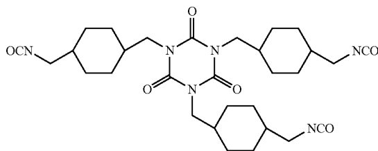
Polyfunctional isocyanate
