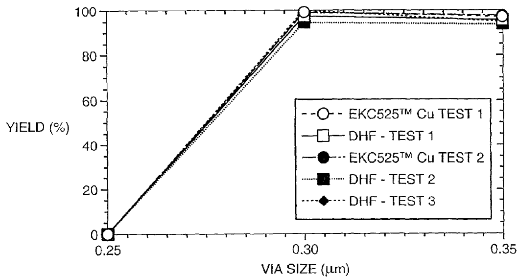
FIG. 38 YIELD RESULTS ON COPPER TEOS STRUCTURE VERSUS VIA SIZE COMPARING DHF AND CLEANING SOLUTION
