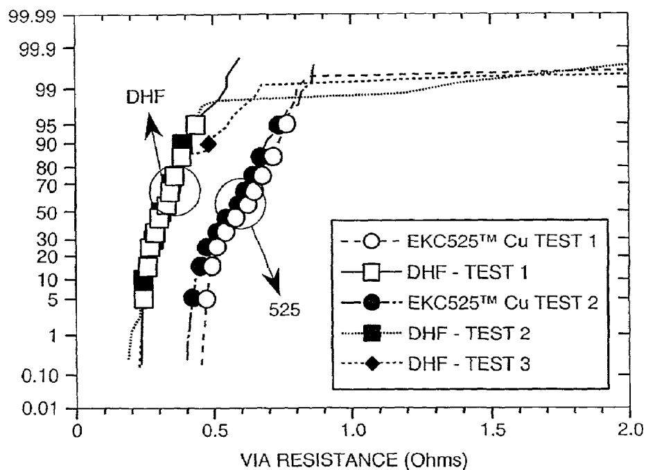
FIG. 39 VIA RESISTANCE HISTOGRAM FOR 0.3 μm VIAS COMPARING DHF AND CLEANING SOLUTION
