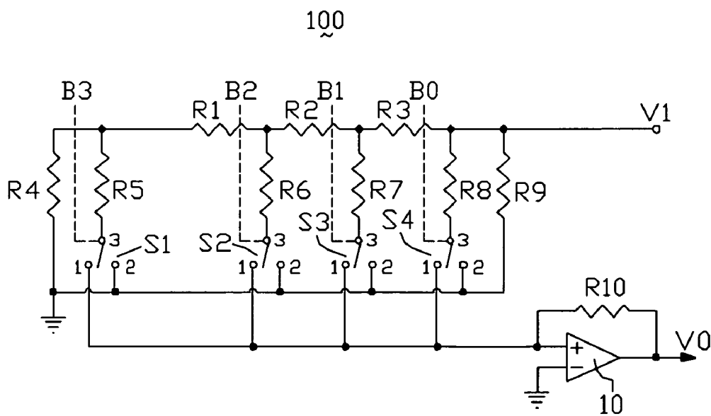
FIG. 2 (RELATED ART)
