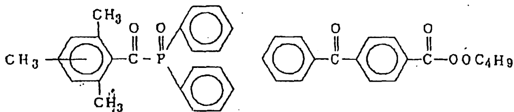
Acylphosphine oxide
