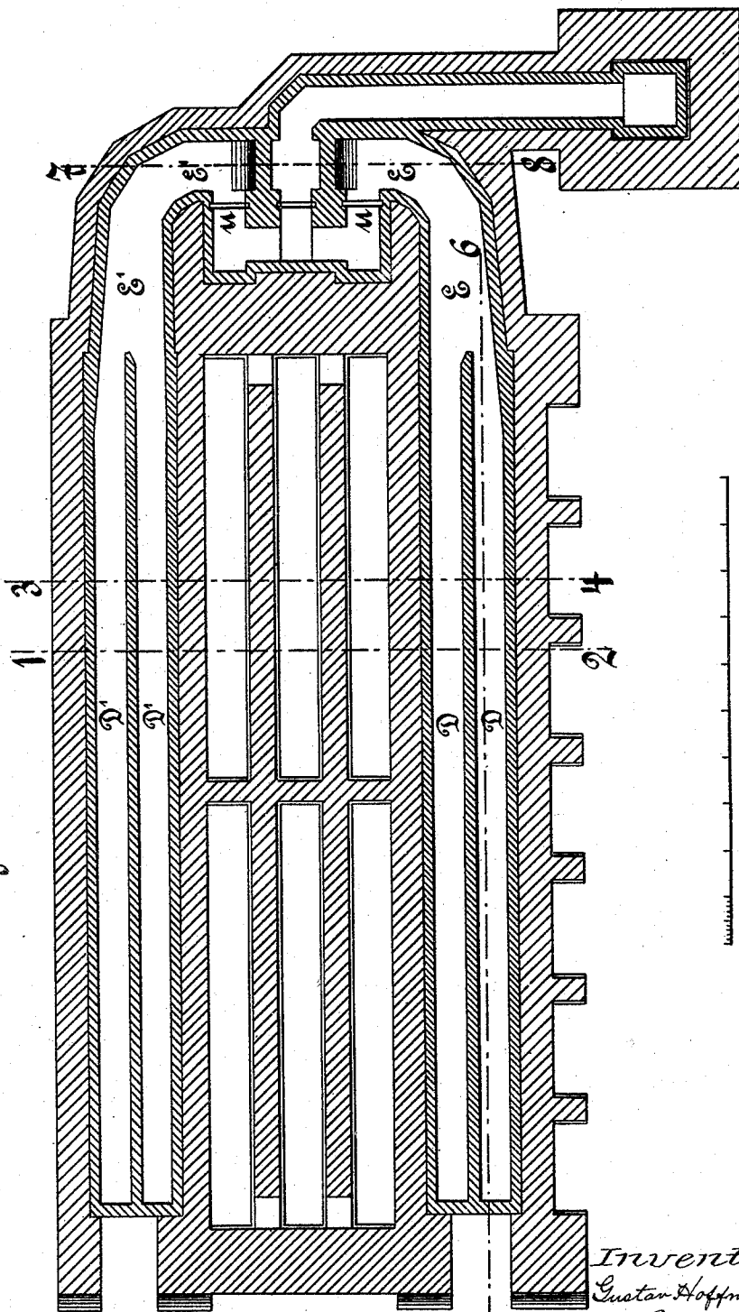
Fig. 5. Section 11-12.
