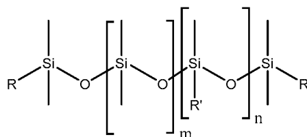
Siloxane Oligomers
