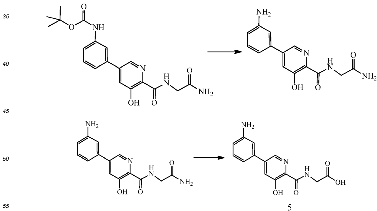
Scheme IV
