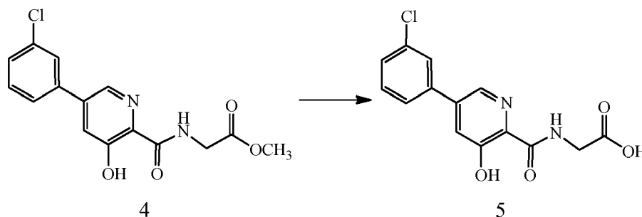
Scheme II
