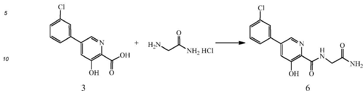
Scheme III
