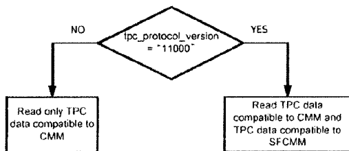
(c) TPC decoding process of SFCMM Receivers
