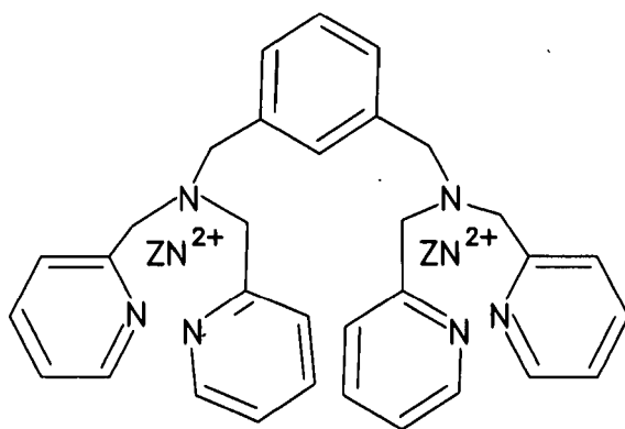
\text{Zn}^{2+} -dipicolylamine Compound 5
