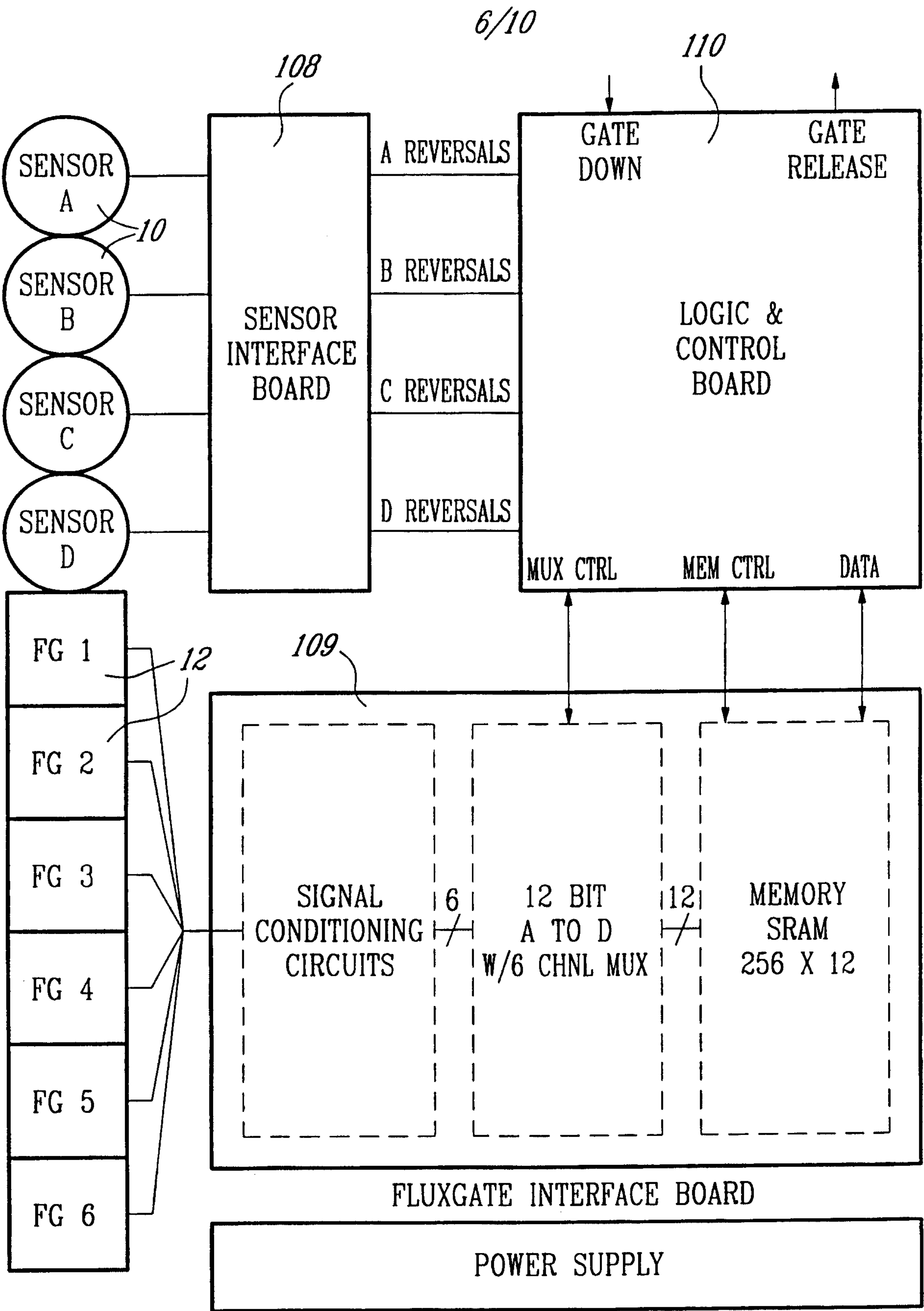
Fig. 5 - 5 ADJUNCT SYSTEM BLOCK DIAGRAM
