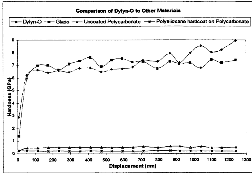
Figure 2: Comparison of Hardness of the coating with uncoated polycarbonate, bare glass and polysiloxane dip coated polycarbonate.
