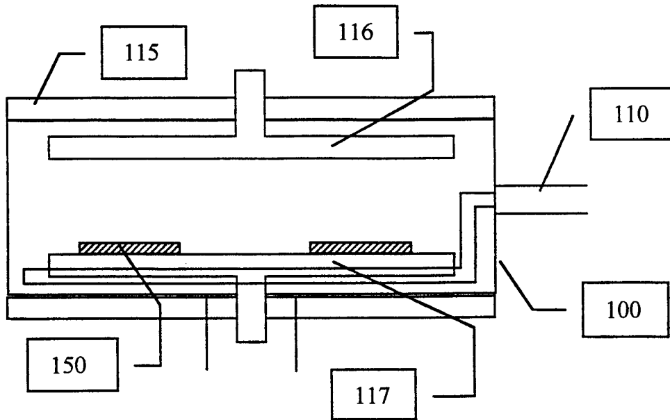
Figure 1: Schematic of a hardcoating deposition chamber.
