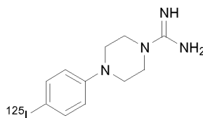
[ 125 I]-1-carboxamidino-4-phenylpiperazine (CAAP)
