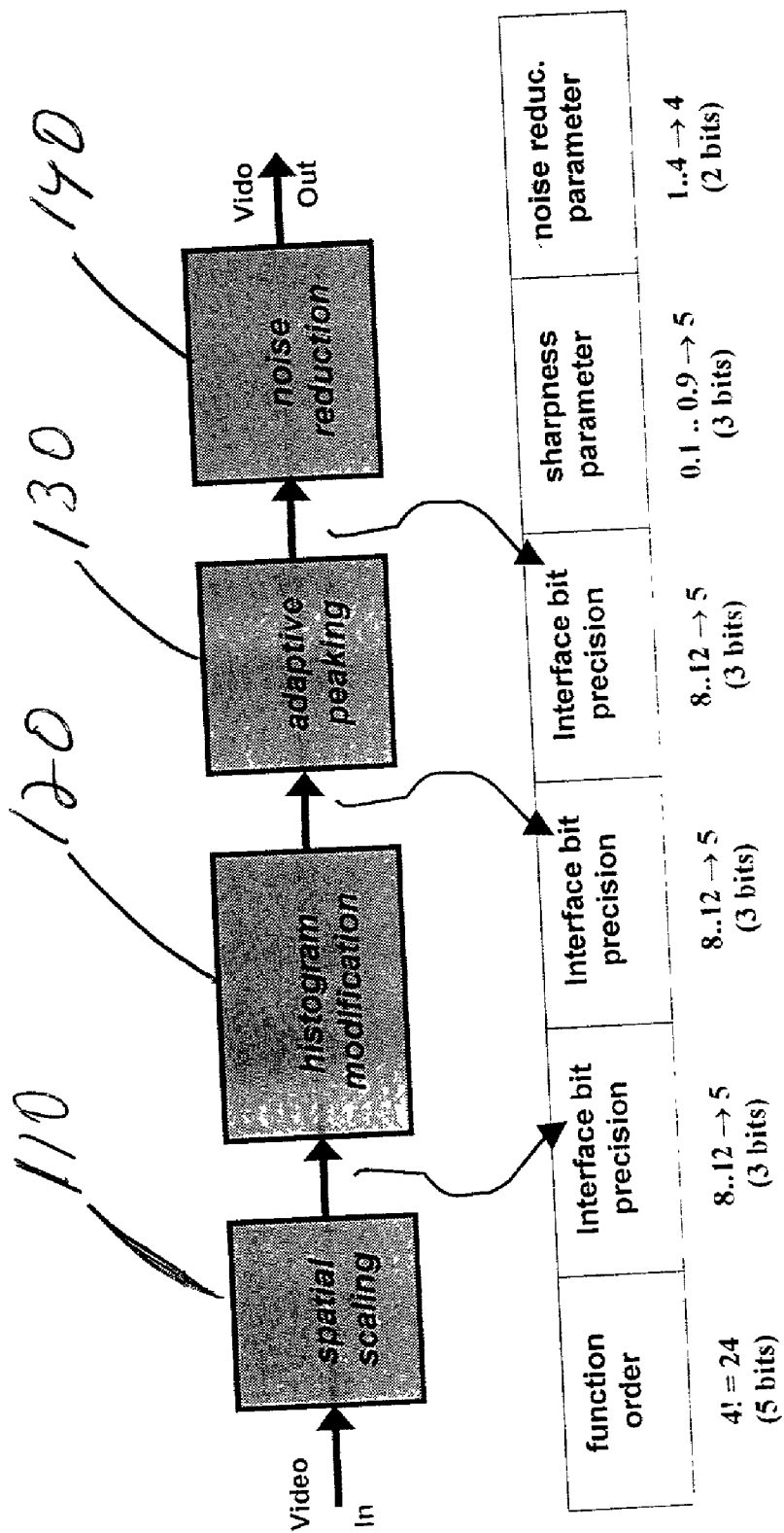
Figure 1 Representing a Video System by a Binary Chromosome
