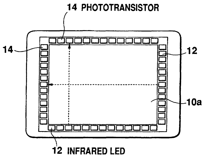
STRUCTURE OF TOUCH PANEL
