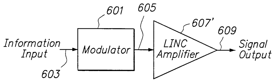
FIG. 6 (PRIOR ART)
