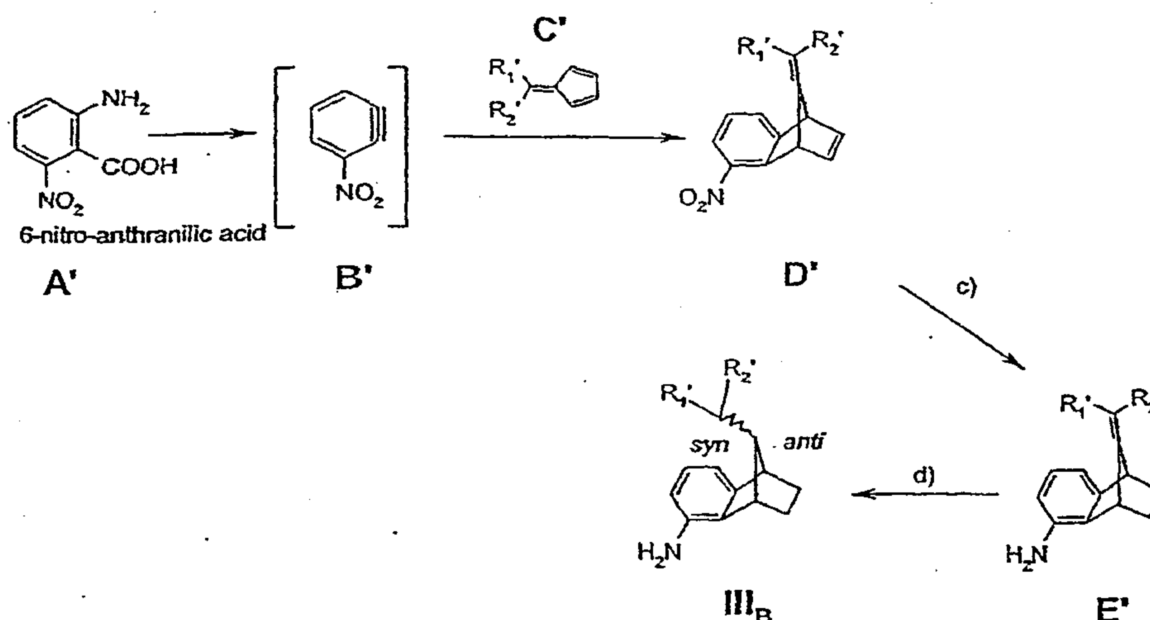
Scheme 1: Synthesis of III B using 6-nitroanthranilic acid
