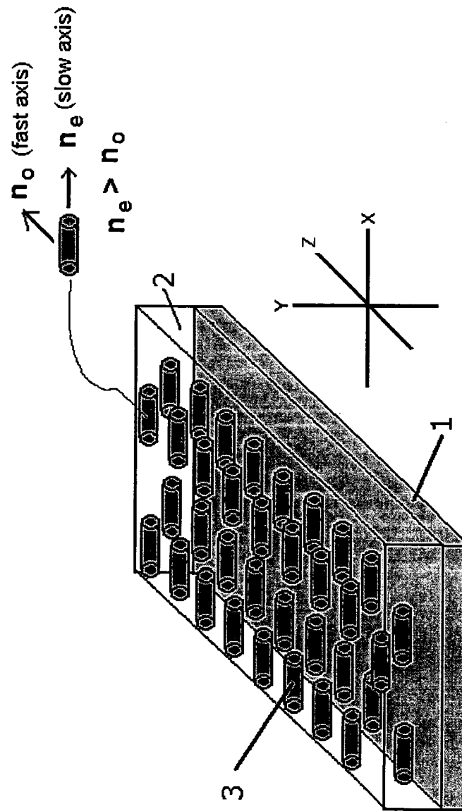
Type A plate
