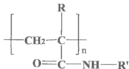
[Chemical Formula 2]
