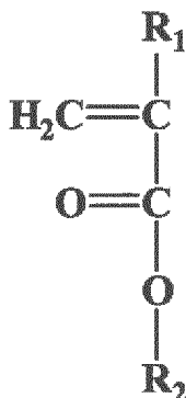
[Chemical Formula 3]
