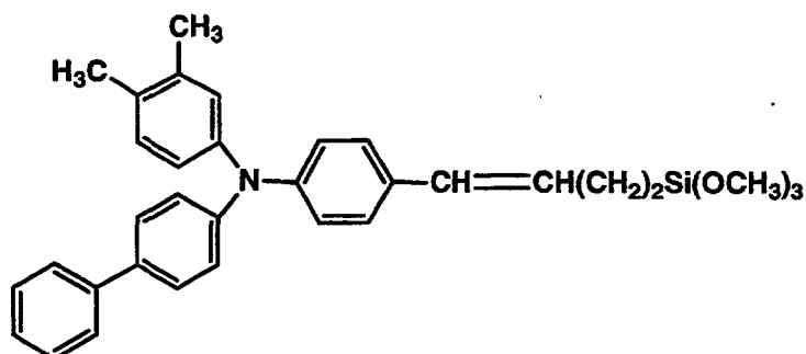
45 Silane compound (A)
