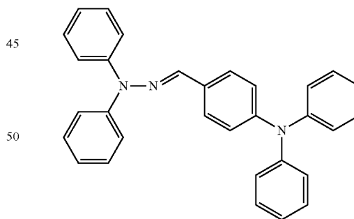
4-(Diphenylamino)benzaldehyde diphenylhydrazone
