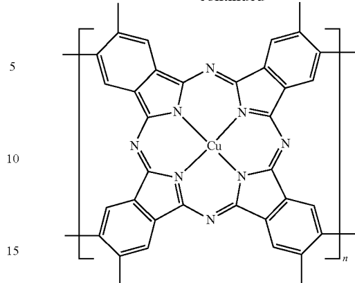
Poly(copper phthalocyanine)
