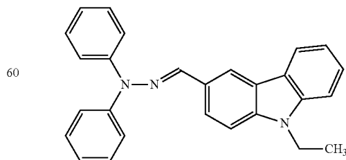
9-Ethyl-3-carbazolecarboxaldehyde diphenylhydrazone
