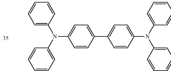
Tetra-N-phenylbenzidine
