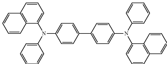
N,N'-Di-[(1-naphthyl)-N,N'-diphenyl]-1,1'-biphenyl-4,4'-diamine
