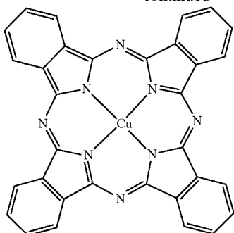
Copper(II) phthalocyanine
