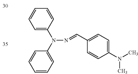
4-(Dimethylamino)benzaldehyde diphenylhydrazone
