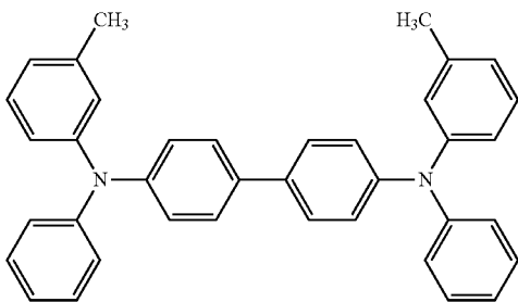
N,N'-Bis(3-methylphenyl)-N,N'-diphenylbenzidine
