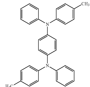
N,N'-Diphenyl-N,N'-di-p-tolylbenzene-1,4-diamine
