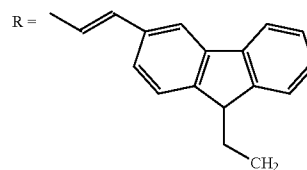
1,3,5-Tris(2-(9-ethylcabazyl-3)ethylene)benzene
