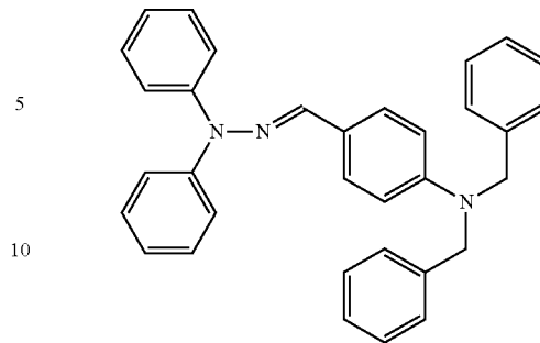
4-(Dibenzylamino)benzaldehyde-N,N-diphenylhydrazone
