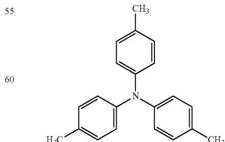
Tri-p-tolylamine
