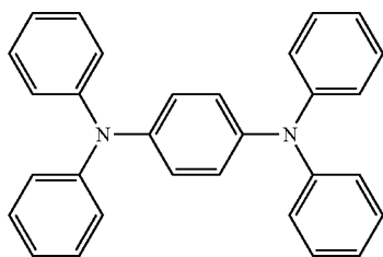
1,4-Bis(diphenylamino)benzene
