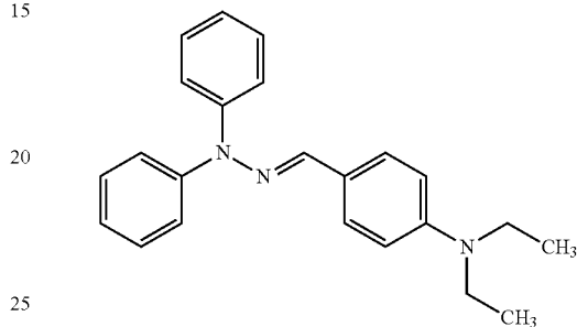
4-(Diethylamino)benzaldehyde diphenylhydrazone
