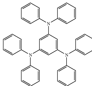
1,3,5-Tris(diphenylamino)benzene
