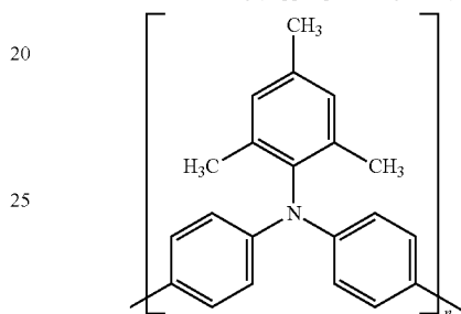
Poly[bis(4-phenyl)(2,4,6-trimethylphenyl)amine]
