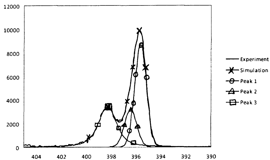
Figure 15: Peak fitting of N 1S region of XPS Spectrum of B150 sample.
