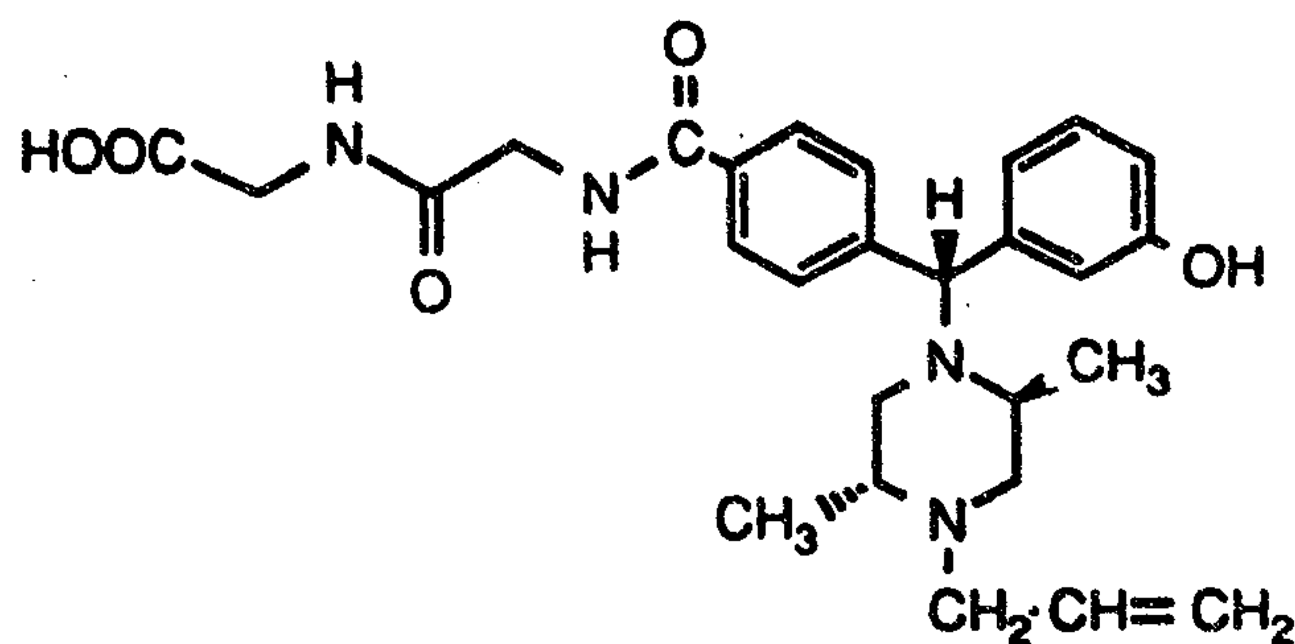
Compound H
