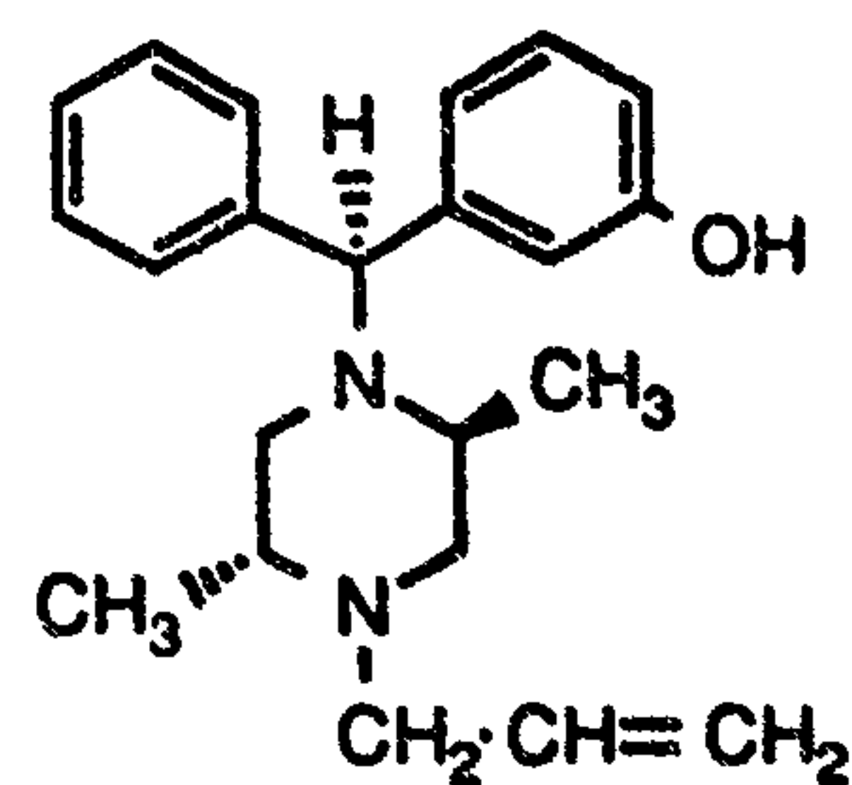
Compound I
