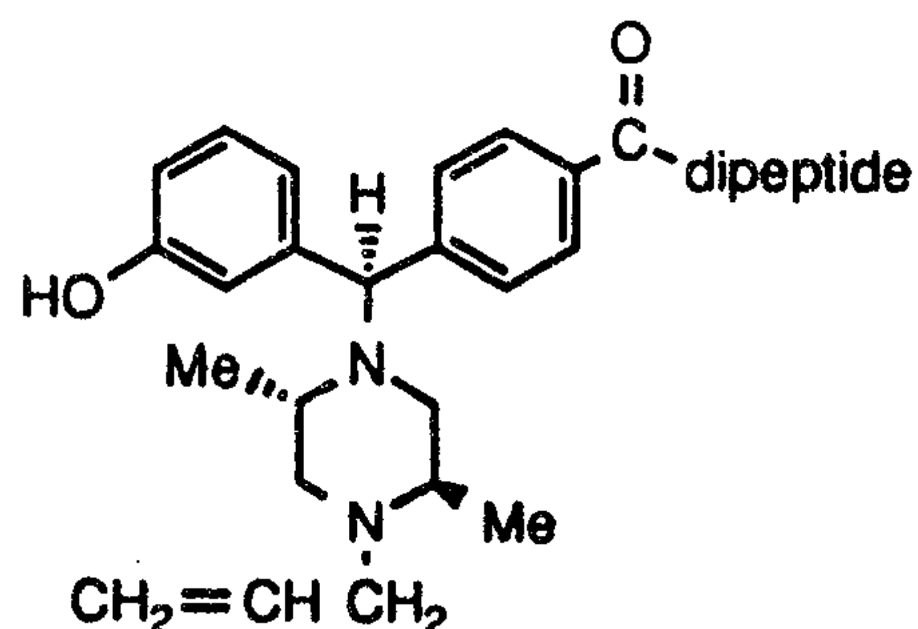
Compound E
