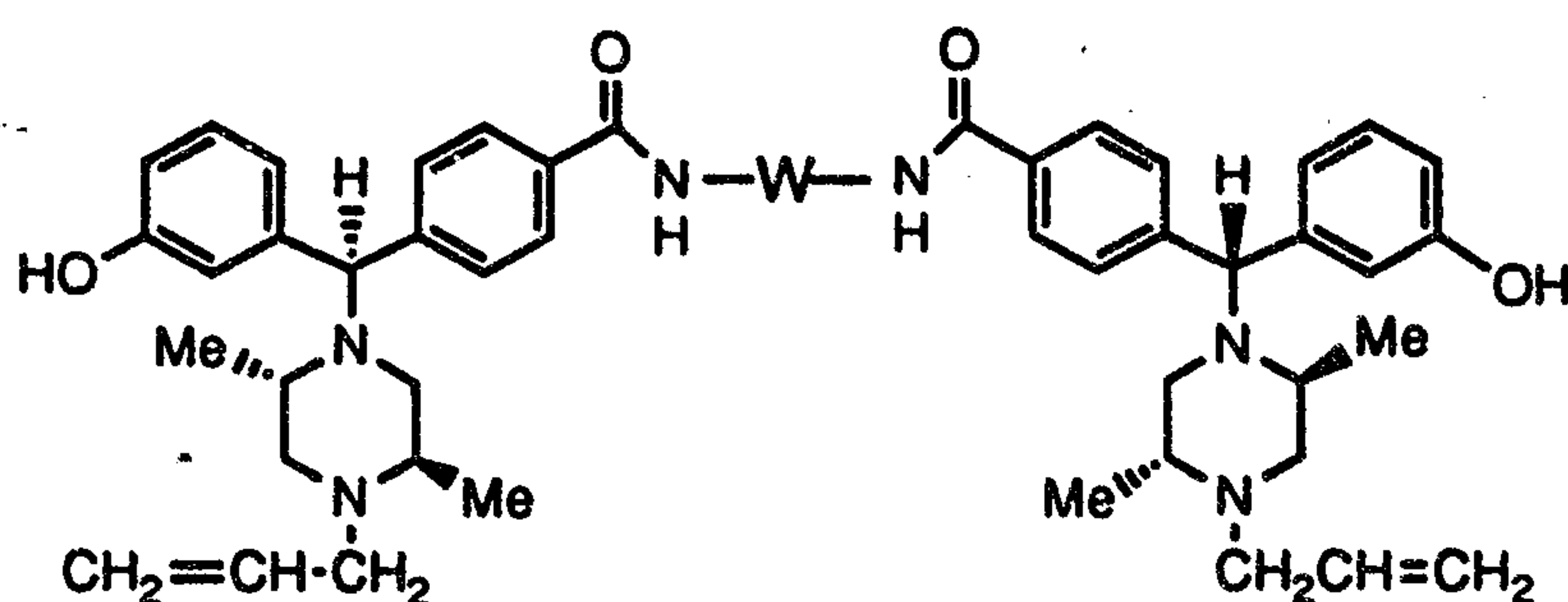
Compound G
