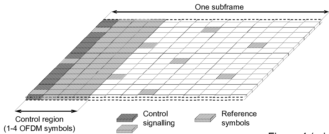
Figure 4 (prior art)
