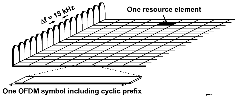
Figure 1 (prior art)
