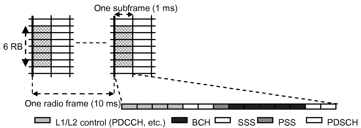
Figure 3 (prior art)
