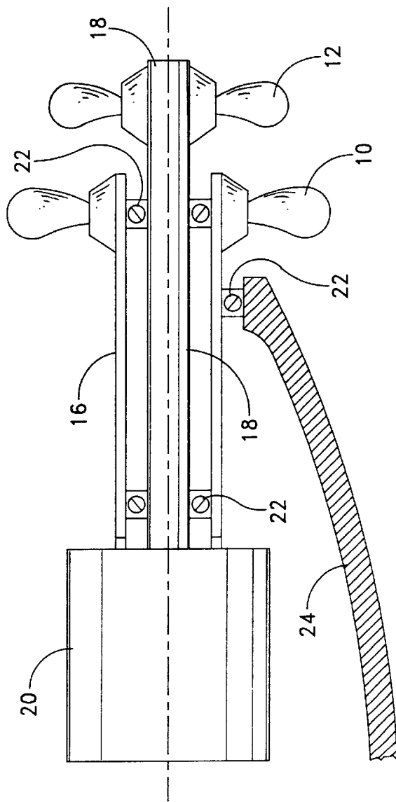
FIG. 2 (PRIOR ART)
