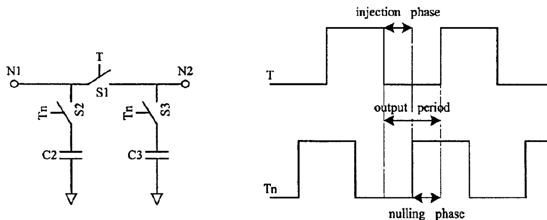
Clocking Sequence Diagram
