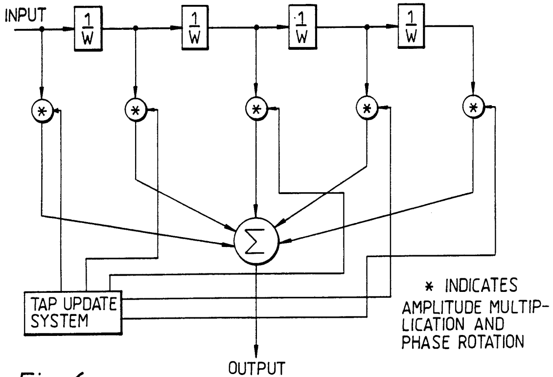
Fig. 6. RAKE DIVERSITY COMBINING SYSTEM
