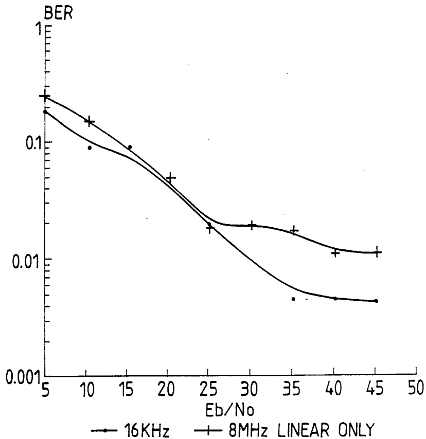
Fig. 8. BER PERFORMANCE NARROW AND WIDEBAND QAM
