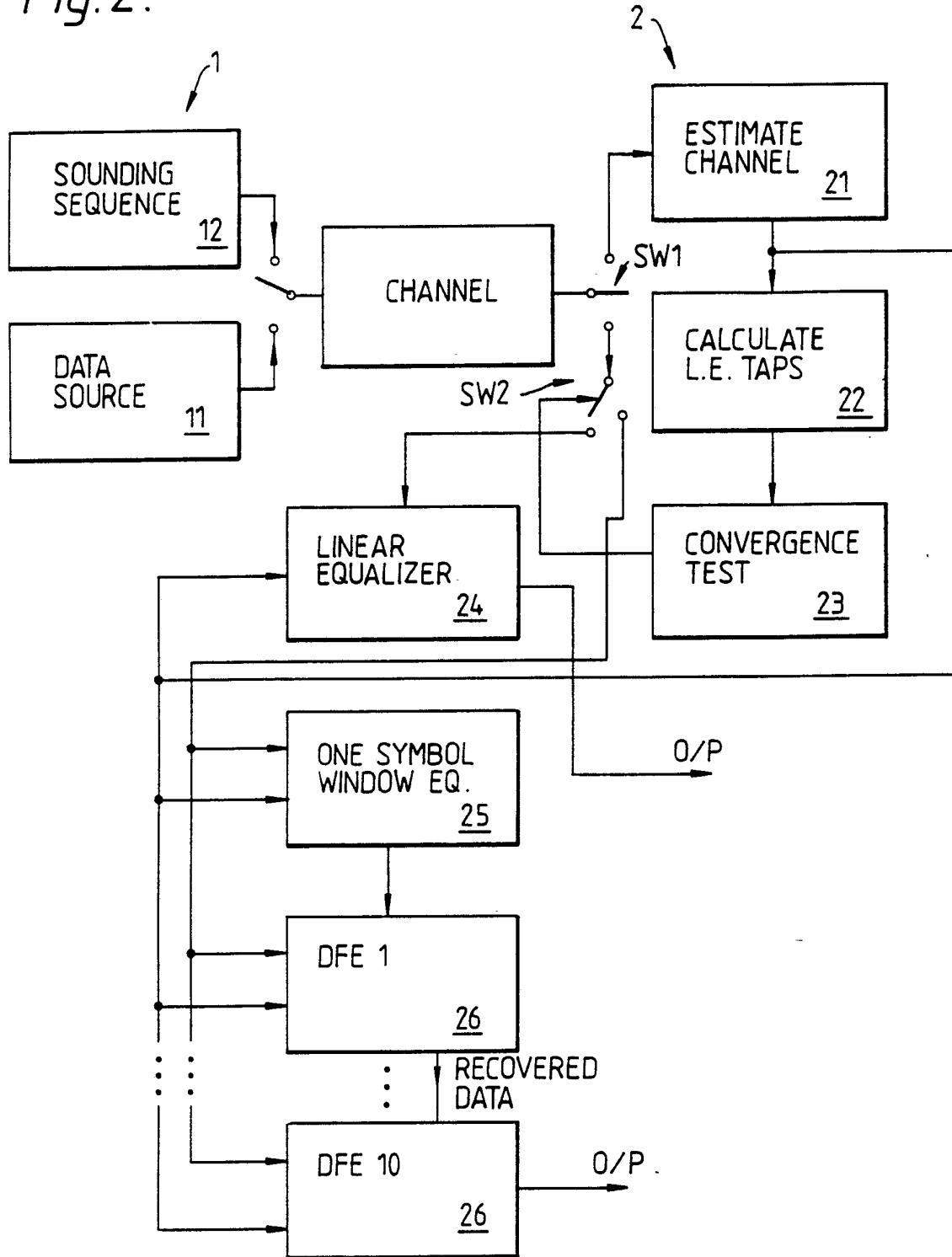
SYSTEM BLOCK DIAGRAM
