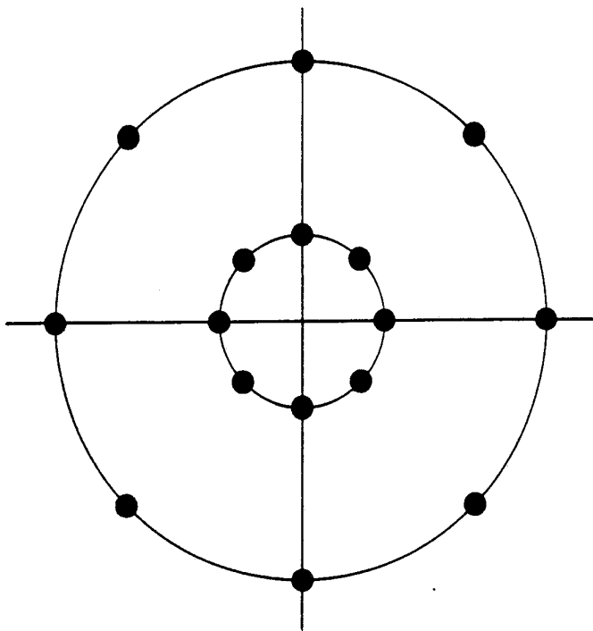
STAR QAM CONSTELLATION
