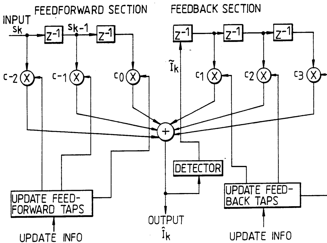
Fig. 5. GENERAL DECISION FEEDBACK EQUALIZER STRUCTURE
