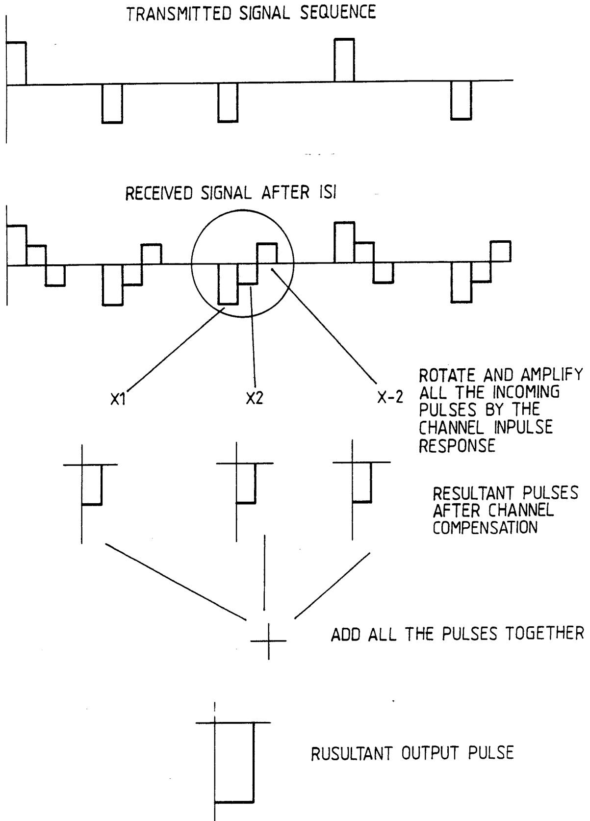
Fig. 7. OPERATION OF THE RAKE COMBINER
