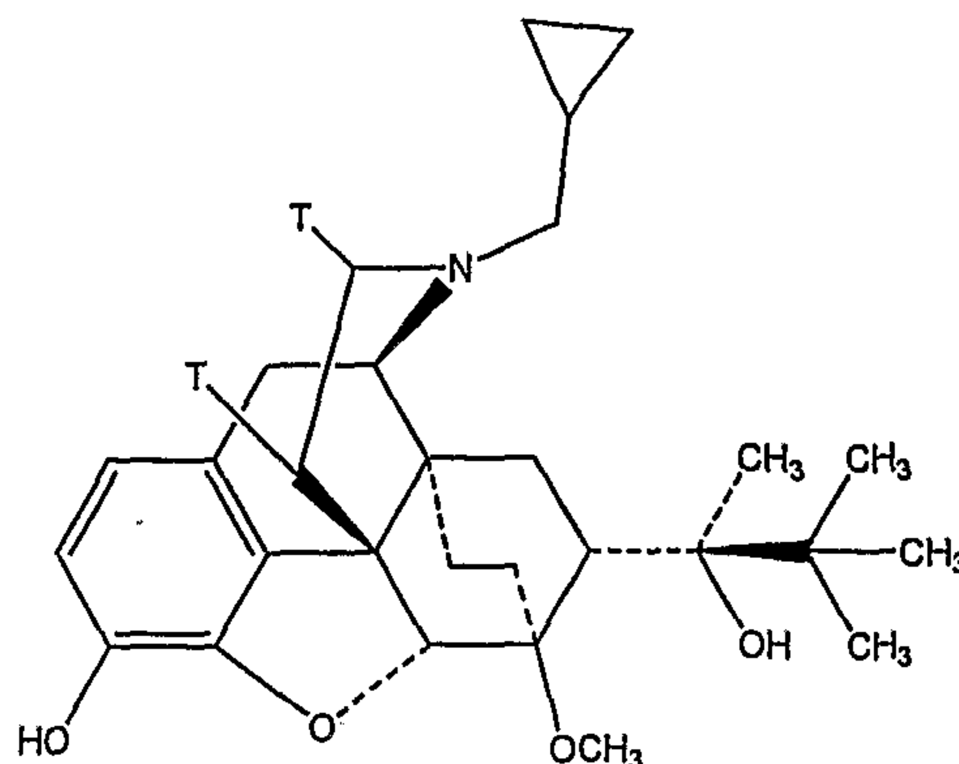
Structure of [15,16- ^3H ] buprenorphine 18 ; T = tritium
