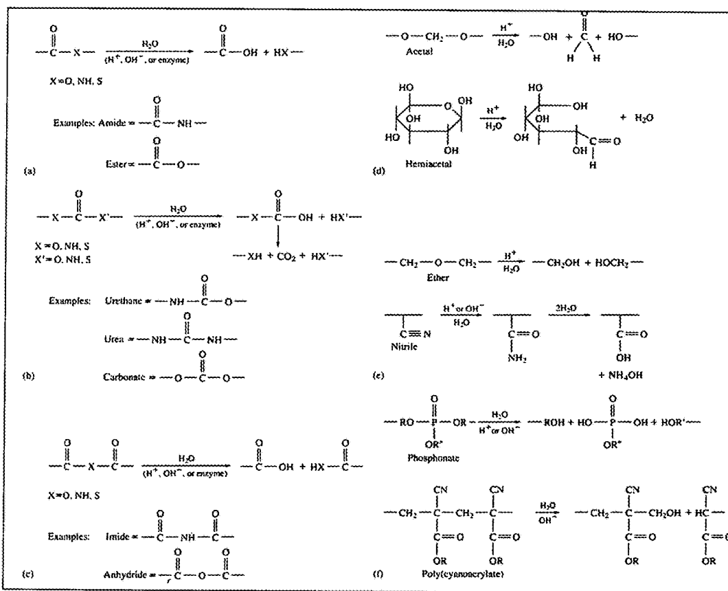
FIG. 1: Hydrolysis Reactions
