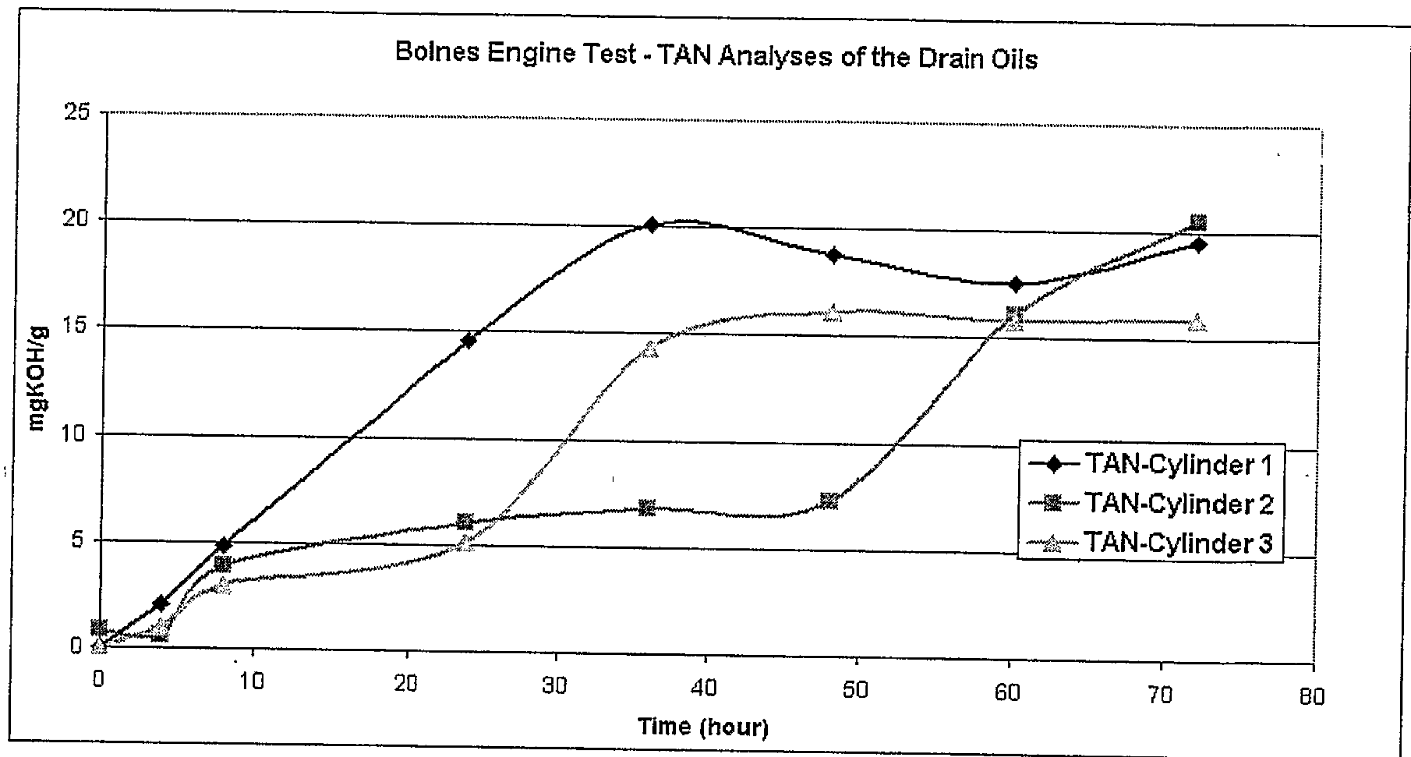
Figure 2: Analyses of the Drain Oils – TAN
