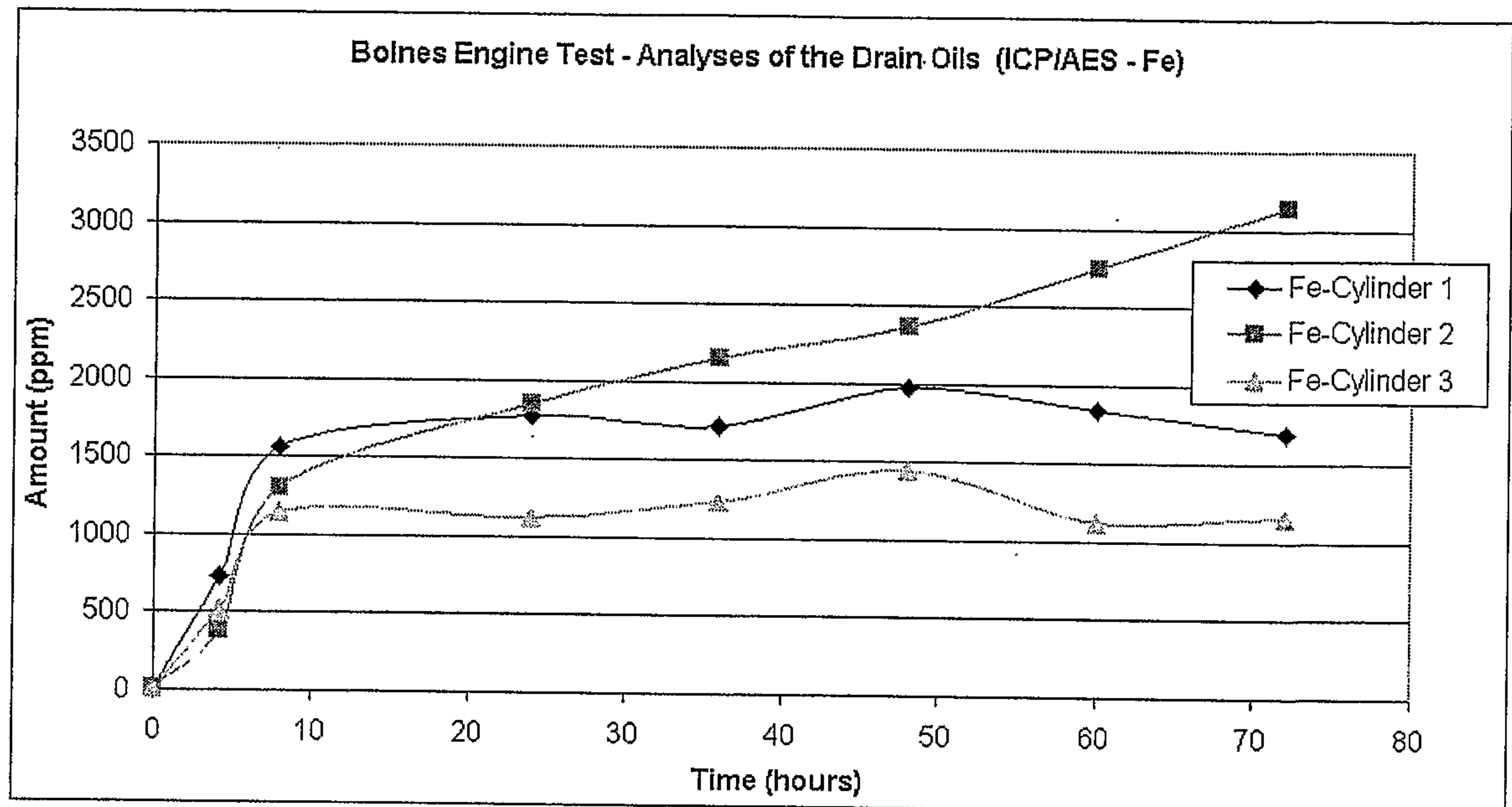
Figure 3: ICP/AES Analyses of the Drain Oils – Fe
