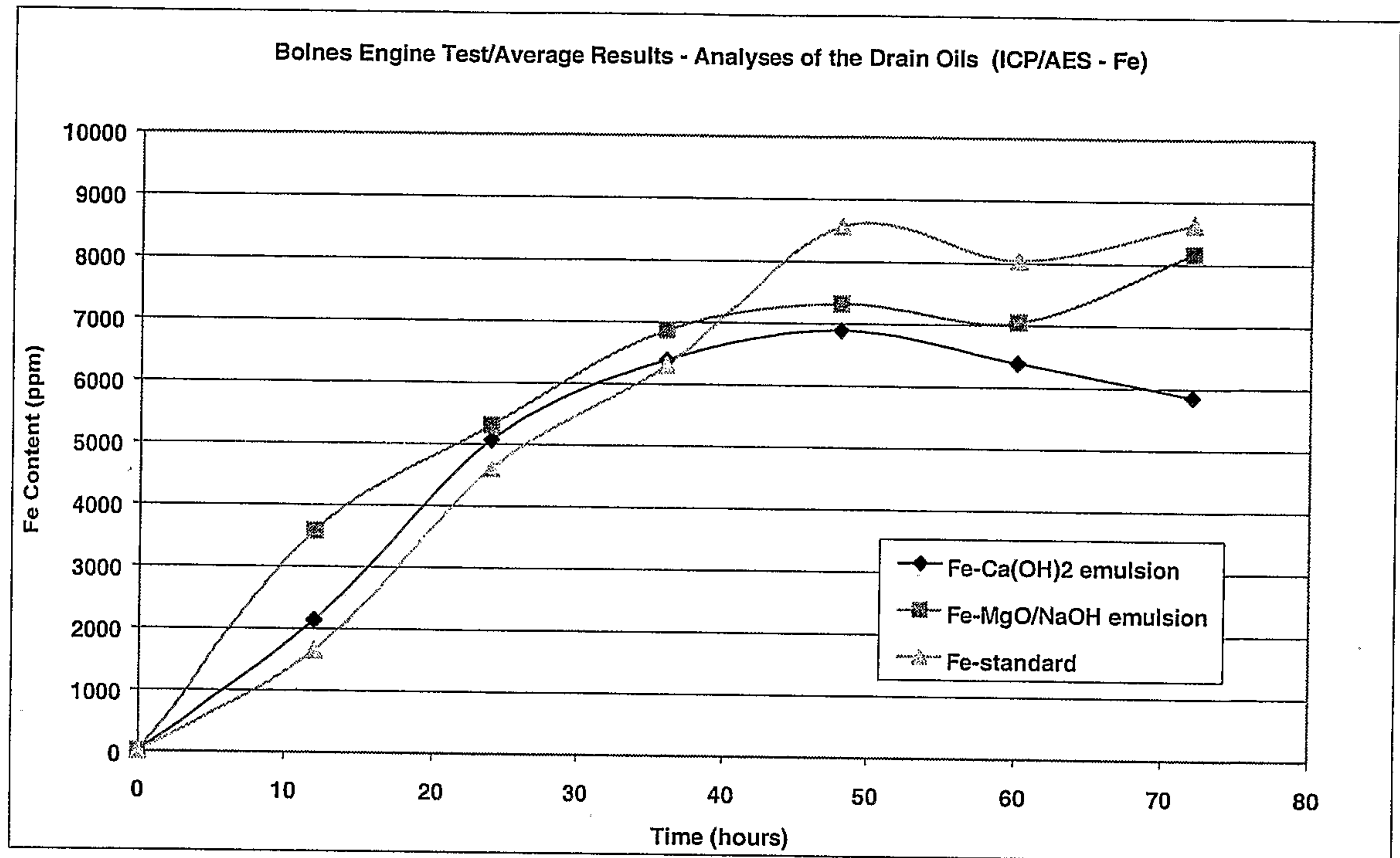
Figure 8: ICP/AES Analyses of the Drain Oils/ – Fe
