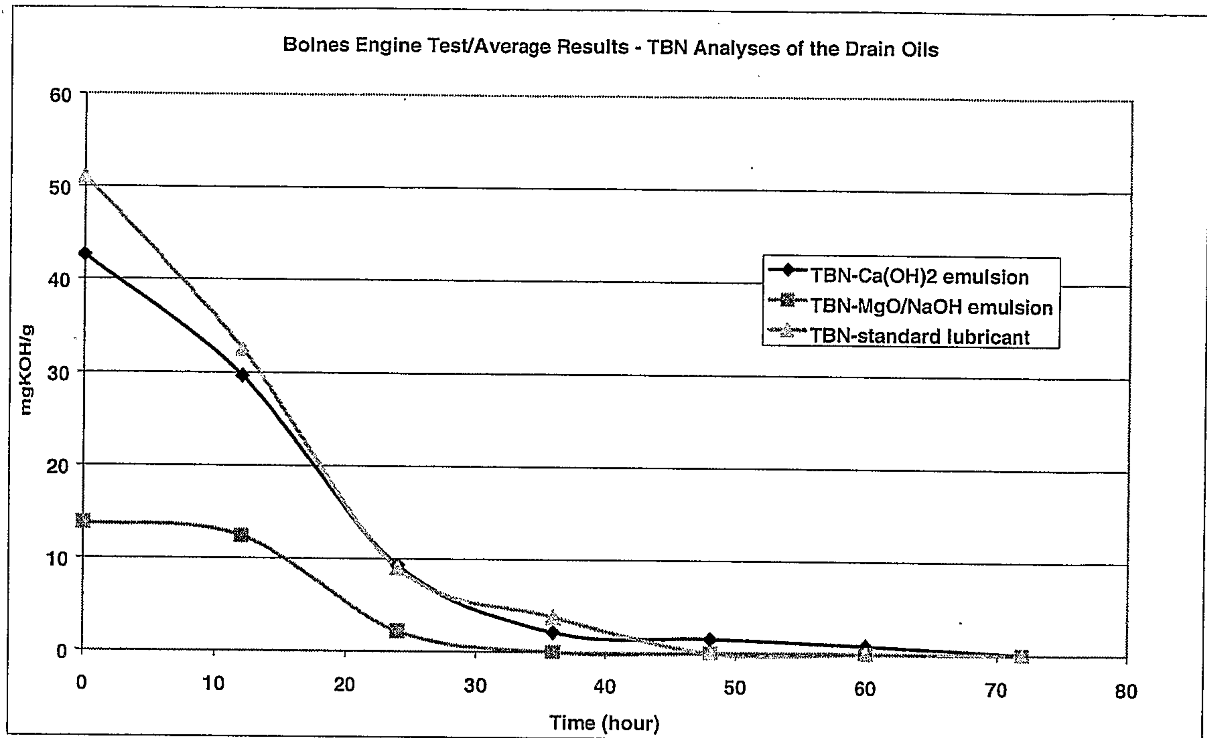
Figure 5: Analyses of the Drain Oils/Average Results – TBN
