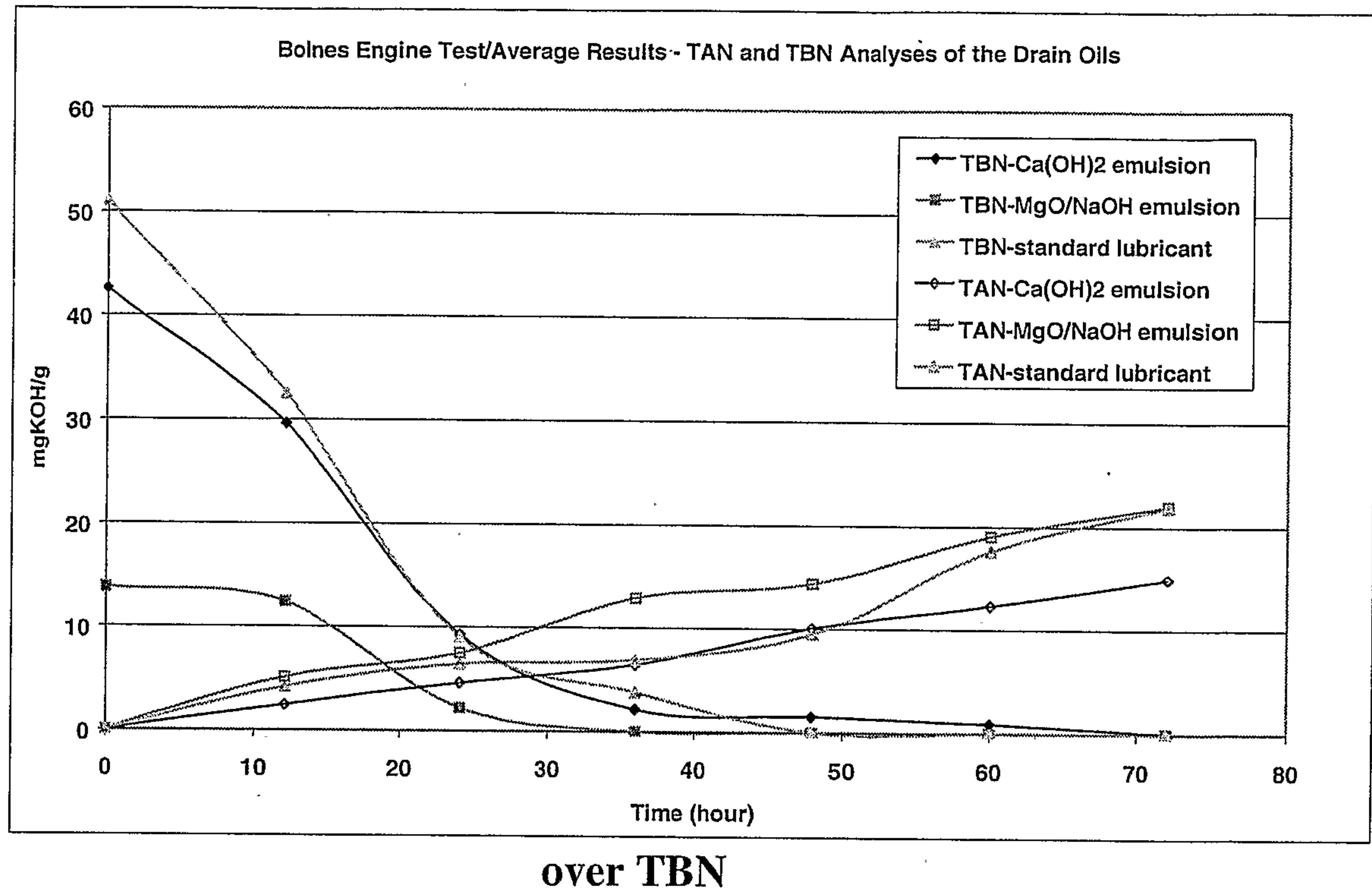
Figure 7: Analyses of the Drain Oils/Average Results – Excess TAN
