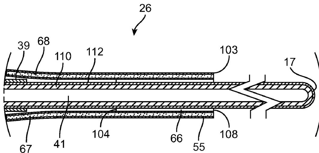
SECTION B-B ROTATED 90°
