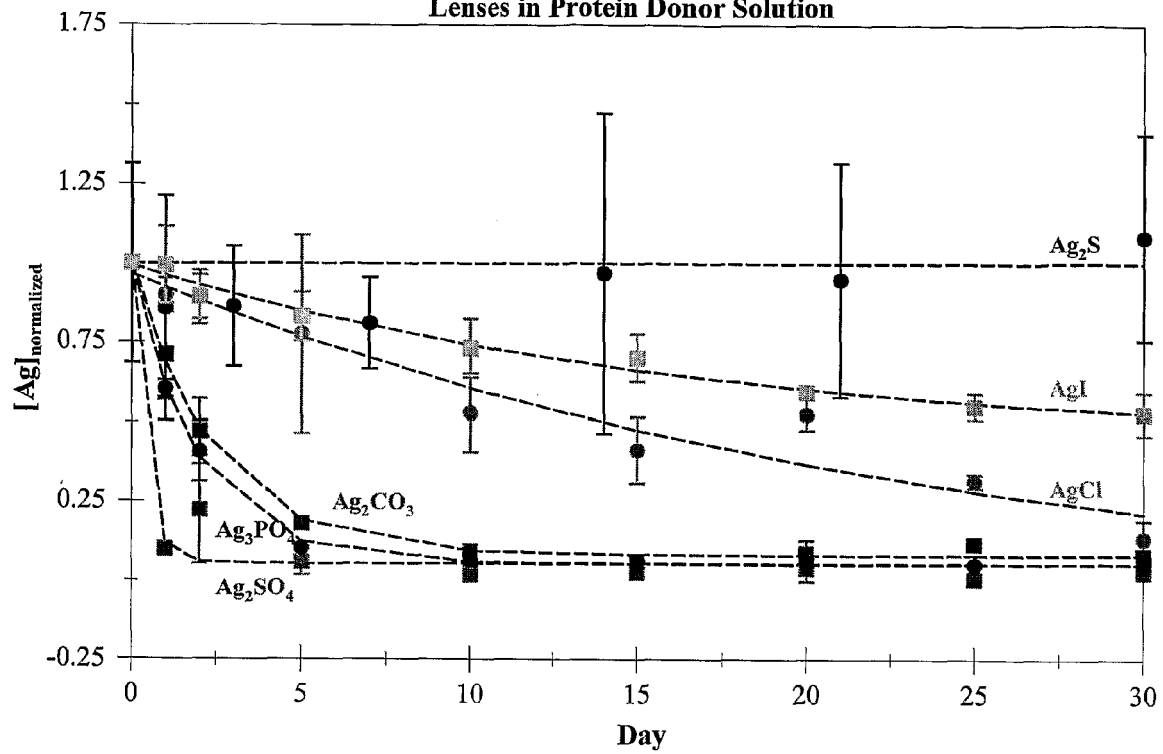
Figure 1. Various Normalized 30/18 y Silver Release Profiles from Contact Lenses in Protein Donor Solution
