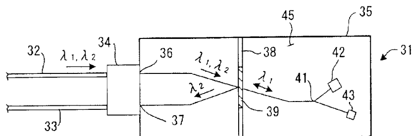
FIG. 3 PRIOR ART
