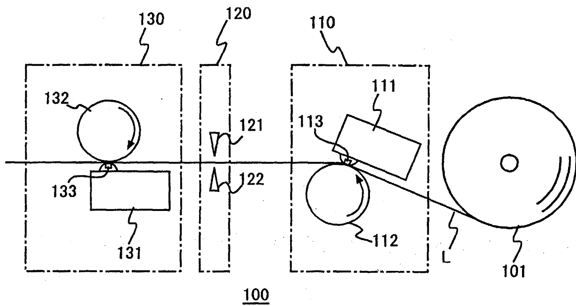
FIG. 6 PRIOR ART
