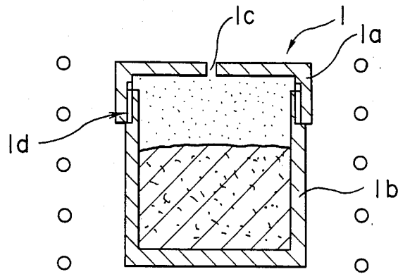
FIG. 5 PRIOR ART
