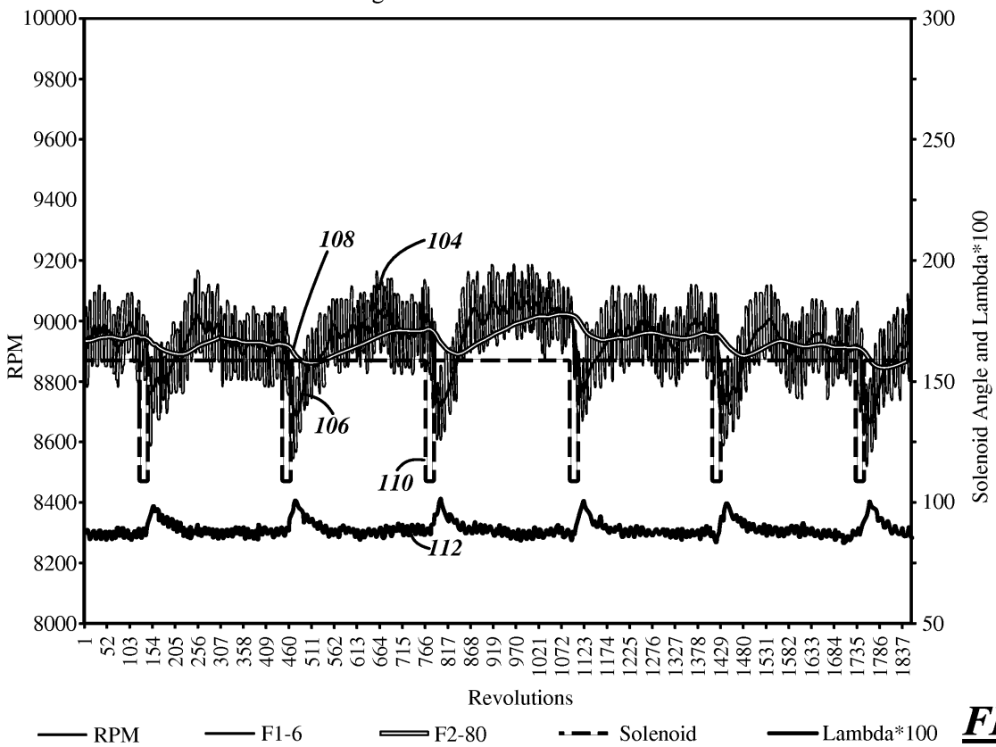
Test 50 Degree Lean 20 Revs Lambda 0.876 Start
