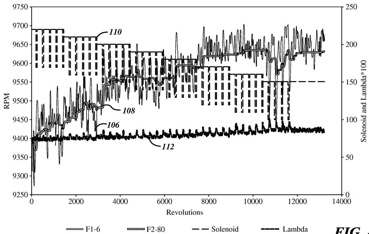
Automatic Adjustment Speed Sensing Test
