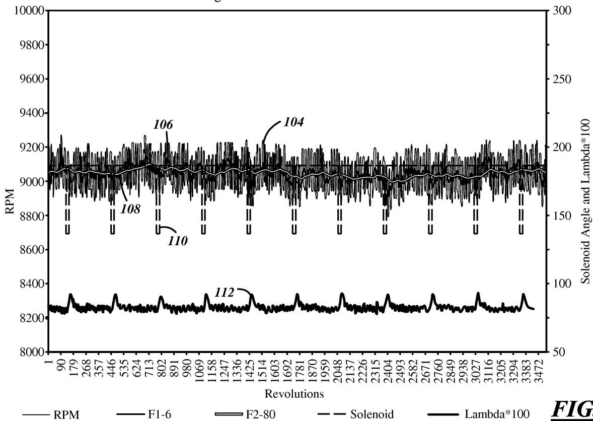
Test 50 Degree Lean 20 Revs Lambda 0.81 Start
