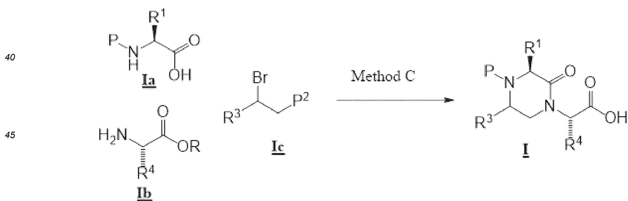
Scheme 3 (Method C)
