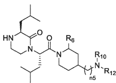
(VIc);
