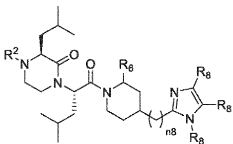
(VIIc);
