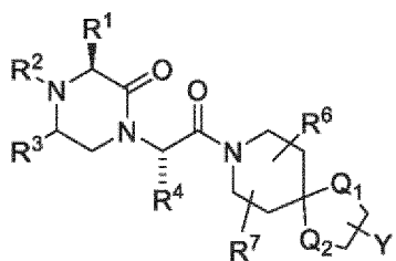
(VIIIc);
