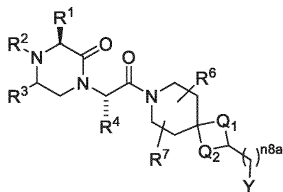
(VIIIa1);
