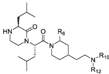
(VIc);
