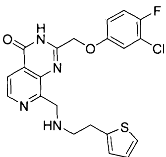
15 2-((3-chloro-4-fluorophenoxy)methyl)-8-(((2-(thiophen-2-yl)ethyl)amino)methyl)pyrido[3,4-d]pyrimidin-4(3H)-one
