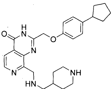
2-((4-cyclopentylphenoxy)methyl)-8-(((piperidin-4-ylmethyl)amino)methyl)pyrido[3,4-d]pyrimidin-4(3H)-one
