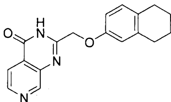
2-(((5,6,7,8-tetrahydronaphthalen-2-yl)oxy)methyl)pyrido[3,4-d]pyrimidin- 4(3H)-one
