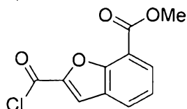
methyl 2-(chlorocarbonyl)benzofuran-7-carboxylate
