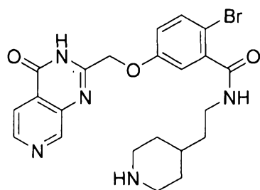
2-bromo-5-((4-oxo-3,4-dihydropyrido[3,4-d]pyrimidin-2-yl)methoxy)-N-(2-(piperidin-4-yl)ethyl)benzamide
