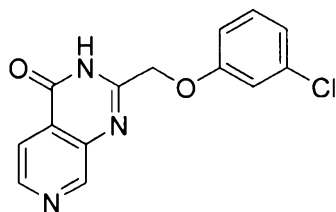
2-((3-chlorophenoxy)methyl)pyrido[3,4-d]pyrimidin-4(3H)-one
