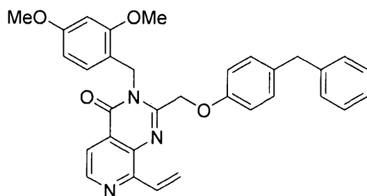
2-((4-benzylphenoxy)methyl)-3-(2,4-dimethoxybenzyl)-8-vinylpyrido[3,4-d]pyrimidin-4(3H)-one
