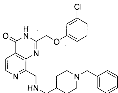
8-((((1-benzylpiperidin-4-yl)methyl)amino)methyl)-2-((3-chlorophenoxy)methyl)pyrido[3,4-d]pyrimidin-4(3H)-one
