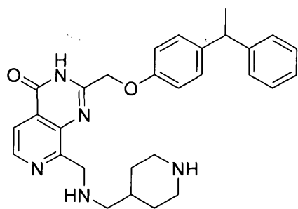
2-((4-(1-phenylethyl)phenoxy)methyl)-8-(((piperidin-4-ylmethyl)amino)methyl)pyrido[3,4-d]pyrimidin-4(3H)-one
