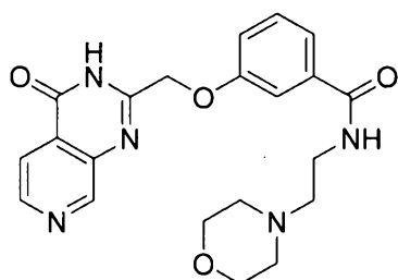
N-(2-morpholinoethyl)-3-((4-oxo-3,4-dihydropyrido[3,4-d]pyrimidin-2-yl)methoxy)benzamide
