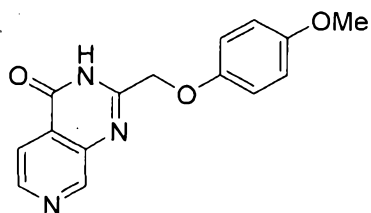
2-((4-methoxyphenoxy)methyl)pyrido[3,4-d]pyrimidin-4(3H)-one
