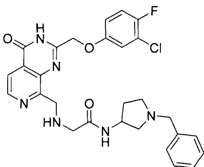
N-(1-benzylpyrrolidin-3-yl)-2-(((2-((3-chloro-4-fluorophenoxy)methyl)-4-oxo-3,4-dihydropyrido[3,4-d]pyrimidin-8-yl)methyl)amino)acetamide
