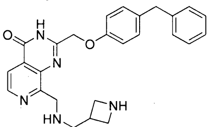
8-(((azetidin-3-ylmethyl)amino)methyl)-2-((4-benzylphenoxy)methyl)pyrido[3,4-d]pyrimidin-4(3H)-one
