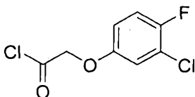
2-(3-chloro-4-fluorophenoxy)acetyl chloride
