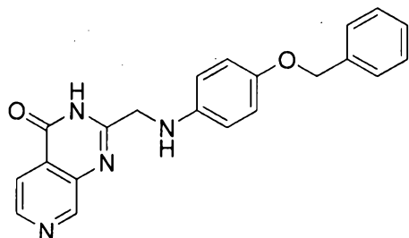
2-(((4-(benzyloxy)phenyl)amino)methyl)pyrido[3,4-d]pyrimidin-4(3H)-one
