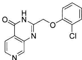
2-((2-chlorophenoxy)methyl)pyrido[3,4-d]pyrimidin-4(3H)-one
