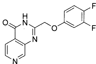
2-((3,4-difluorophenoxy)methyl)pyrido[3,4-d]pyrimidin-4(3H)-one
