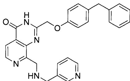
2-((4-benzylphenoxy)methyl)-8-(((pyridin-3-ylmethyl)amino)methyl)pyrido[3,4-d]pyrimidin-4(3H)-one
