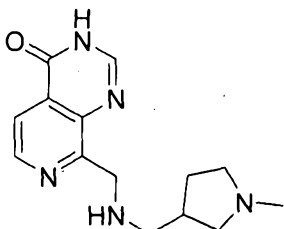
8-(((1-methylpyrrolidin-3-yl)methyl)amino)methyl)pyrido[3,4-d]pyrimidin- 4(3H)-one
