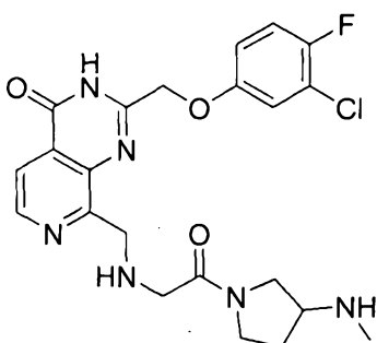
2-((3-chloro-4-fluorophenoxy)methyl)-8-(((2-(3-(methylamino)pyrrolidin-1-yl)-2-oxoethyl)amino)methyl)pyrido[3,4-d]pyrimidin-4(3H)-one
