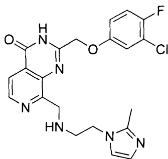
2-((3-chloro-4-fluorophenoxy)methyl)-8-(((2-(2-methyl-1H-imidazol-1-yl)ethyl)amino)methyl)pyrido[3,4-d]pyrimidin-4(3H)-one
