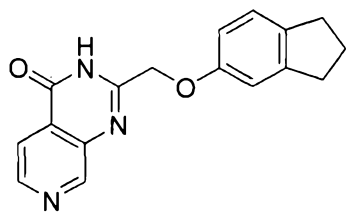
2-(((2,3-dihydro-1H-inden-5-yl)oxy)methyl)pyrido[3,4-d]pyrimidin-4(3H)-one
