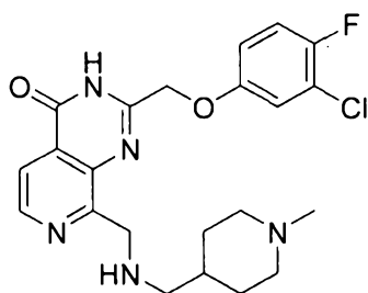
2-((3-chloro-4-fluorophenoxy)methyl)-8-((((1-methylpiperidin-4-yl)methyl)amino)methyl)pyrido[3,4-d]pyrimidin-4(3H)-one
