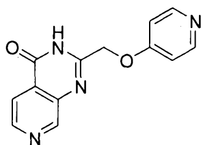
2-((pyridin-4-yloxy)methyl)pyrido[3,4-d]pyrimidin-4(3H)-one
