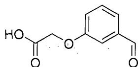
2-(3-formylphenoxy)acetic acid
