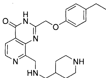
2-((4-ethylphenoxy)methyl)-8-(((piperidin-4-ylmethyl)amino)methyl)pyrido[3,4-d]pyrimidin-4(3H)-one
