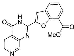
methyl 2-(4-oxo-3,4-dihydropyrido[3,4-d]pyrimidin-2-yl)benzofuran-7-carboxylate
