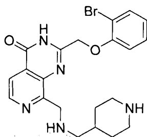
2-((2-bromophenoxy)methyl)-8-(((piperidin-4-ylmethyl)amino)methyl)pyrido[3,4-d]pyrimidin-4(3H)-one
