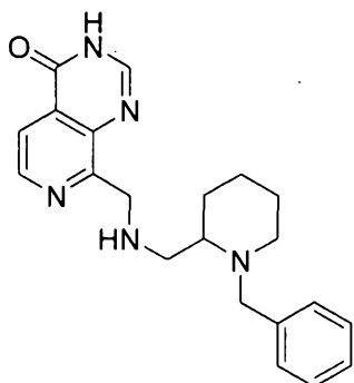
8-((((1-benzylpiperidin-2-yl)methyl)amino)methyl)pyrido[3,4-d]pyrimidin-4(3H)-one
