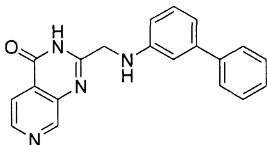
2-(((1,1'-biphenyl)-3-ylamino)methyl)pyrido[3,4-d]pyrimidin-4(3H)-one
