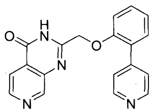
2-((2-(pyridin-4-yl)phenoxy)methyl)pyrido[3,4-d]pyrimidin-4(3H)-one
