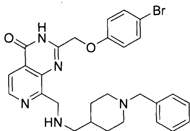
8-((((1-benzylpiperidin-4-yl)methyl)amino)methyl)-2-((4-bromophenoxy)methyl)pyrido[3,4-d]pyrimidin-4(3H)-one
