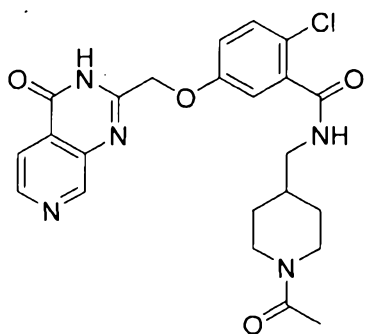
N-((1-acetylpiperidin-4-yl)methyl)-2-chloro-5-((4-oxo-3,4-dihydropyrido[3,4-d]pyrimidin-2-yl)methoxy)benzamide
