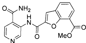
methyl 2-((4-carbamoylpyridin-3-yl)carbamoyl)benzofuran-7-carboxylate
