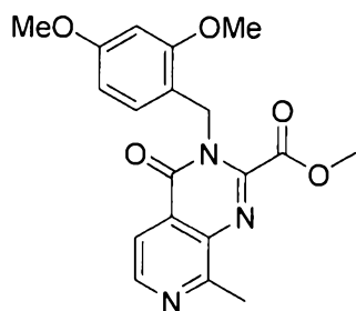
methyl 3-(2,4-dimethoxybenzyl)-8-methyl-4-oxo-3,4-dihydropyrido[3,4-d]pyrimidine-2-carboxylate
