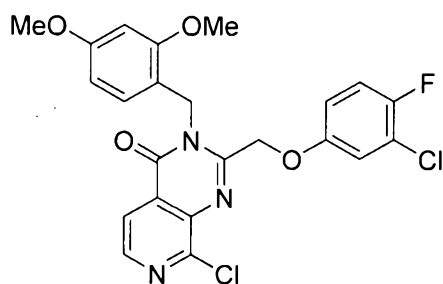
8-chloro-2-((3-chloro-4-fluorophenoxy)methyl)-3-(2,4-dimethoxybenzyl)pyrido[3,4-d]pyrimidin-4(3H)-one
