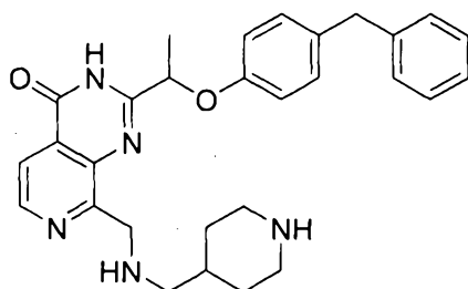
2-(1-(4-benzylphenoxy)ethyl)-8-(((piperidin-4-ylmethyl)amino)methyl)pyrido[3,4-d]pyrimidin-4(3H)-one
