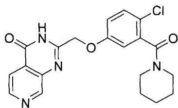
2-((4-chloro-3-(piperidine-1-carbonyl)phenoxy)methyl)pyrido[3,4-d]pyrimidin-4(3H)-one
