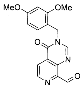
3-(2,4-dimethoxybenzyl)-4-oxo-3,4-dihydropyrido[3,4-d]pyrimidine-8-carbaldehyde
