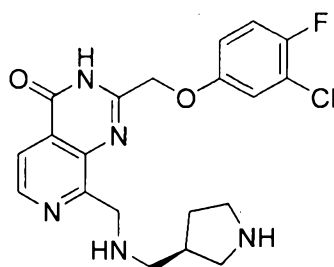
(S)-2-((3-chloro-4-fluorophenoxy)methyl)-8-(((pyrrolidin-3-ylmethyl)amino)methyl)pyrido[3,4-d]pyrimidin-4(3H)-one
