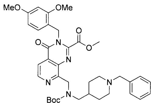
methyl 8-((((1-benzylpiperidin-4-yl)methyl)(tert-butoxycarbonyl)amino)methyl)-3-(2,4-dimethoxybenzyl)-4-oxo-3,4-dihydropyrido[3,4-d]pyrimidine-2-carboxylate
