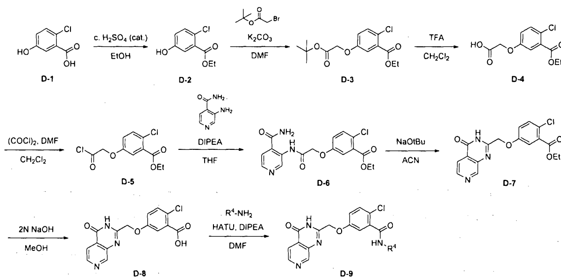
Scheme 4 (Method D)
