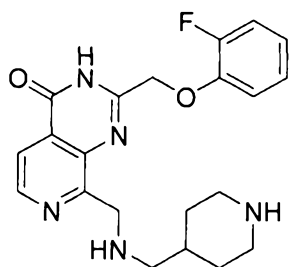
2-((2-fluorophenoxy)methyl)-8-(((piperidin-4-ylmethyl)amino)methyl)pyrido[3,4-d]pyrimidin-4(3H)-one
