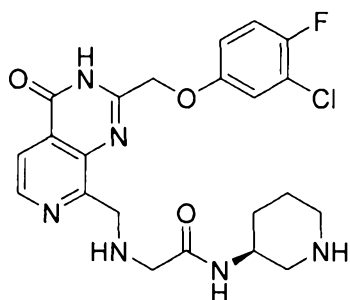
(S)-2-(((2-((3-chloro-4-fluorophenoxy)methyl)-4-oxo-3,4-dihydropyrido[3,4-d]pyrimidin-8-yl)methyl)amino)-N-(piperidin-3-yl)acetamide
