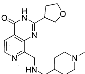
15 8-(((1-methylpiperidin-4-yl)methyl)amino)methyl)-2-(tetrahydrofuran-3-yl)pyrido[3,4-d]pyrimidin-4(3H)-one
