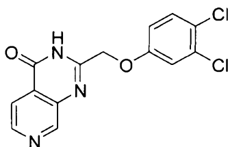
2-((3,4-dichlorophenoxy)methyl)pyrido[3,4-d]pyrimidin-4(3H)-one
