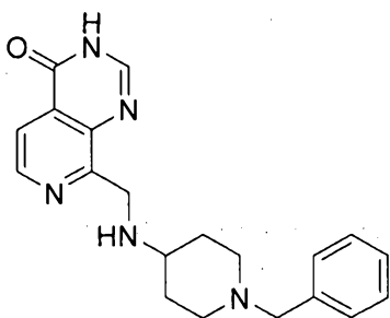
8-((((1-benzylpiperidin-4-yl)amino)methyl)pyrido[3,4-d]pyrimidin-4(3H)-one
