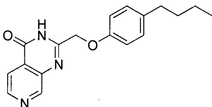
2-((4-butylphenoxy)methyl)pyrido[3,4-d]pyrimidin-4(3H)-one
