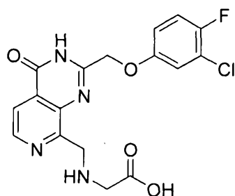
((2-((3-chloro-4-fluorophenoxy)methyl)-4-oxo-3,4-dihydropyrido[3,4-d]pyrimidin-8-yl)methyl)glycine
