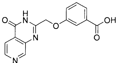
3-((4-oxo-3,4-dihydropyrido[3,4-d]pyrimidin-2-yl)methoxy)benzoate
