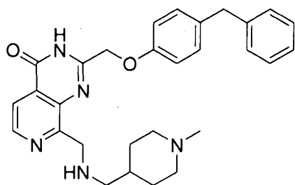
2-((4-benzylphenoxy)methyl)-8-(((1-methylpiperidin-4-yl)methyl)amino)methyl)pyrido[3,4-d]pyrimidin-4(3H)-one
