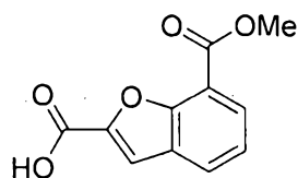
7-(methoxycarbonyl)benzofuran-2-carboxylic acid
