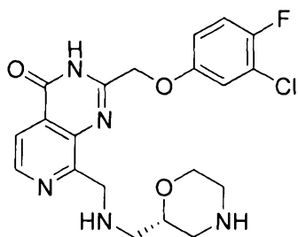
(S)-2-(((3-chloro-4-fluorophenoxy)methyl)-8-(((morpholin-2-ylmethyl)amino)methyl)pyrido[3,4-d]pyrimidin-4(3H)-one
