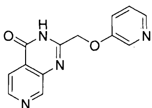
2-((pyridin-3-yloxy)methyl)pyrido[3,4-d]pyrimidin-4(3H)-one
