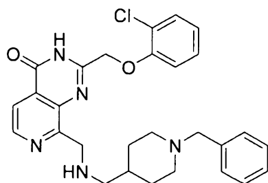
8-((((1-benzylpiperidin-4-yl)methyl)amino)methyl)-2-((2-chlorophenoxy)methyl)pyrido[3,4-d]pyrimidin-4(3H)-one
