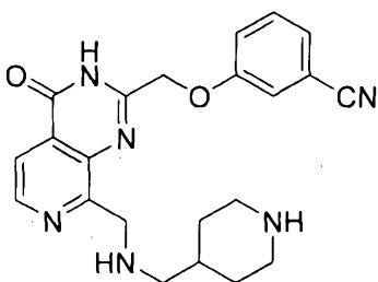
3-((4-oxo-8-(((piperidin-4-ylmethyl)amino)methyl)-3,4-dihydropyrido[3,4-d]pyrimidin-2-yl)methoxy)benzonitrile
