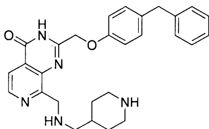
2-((4-benzylphenoxy)methyl)-8-(((piperidin-4-ylmethyl)amino)methyl)pyrido[3,4-d]pyrimidin-4(3H)-one
