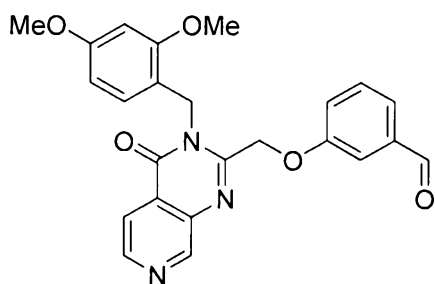
3-((3-(2,4-dimethoxybenzyl)-4-oxo-3,4-dihydropyrido[3,4-d]pyrimidin-2-yl)methoxy)benzaldehyde
