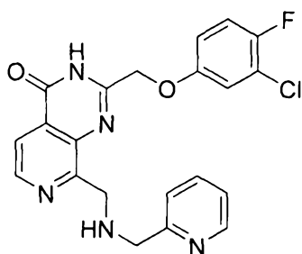
2-((3-chloro-4-fluorophenoxy)methyl)-8-(((pyridin-2-ylmethyl)amino)methyl)pyrido[3,4-d]pyrimidin-4(3H)-one
