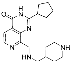
2-cyclopentyl-8-(((piperidin-4-ylmethyl)amino)methyl)pyrido[3,4-d]pyrimidin-4(3H)-one
