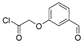
2-(3-formylphenoxy)acetyl chloride
