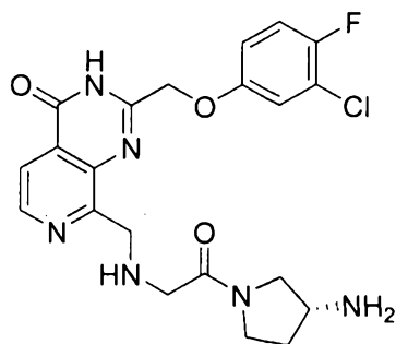
(R)-8-(((2-(3-aminopyrrolidin-1-yl)-2-oxoethyl)amino)methyl)-2-((3-chloro-4-fluorophenoxy)methyl)pyrido[3,4-d]pyrimidin-4(3H)-one
