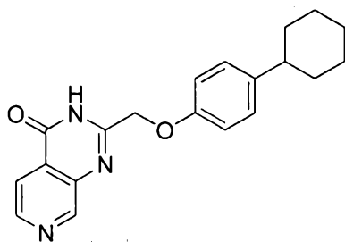
2-((4-cyclohexylphenoxy)methyl)pyrido[3,4-d]pyrimidin-4(3H)-one
