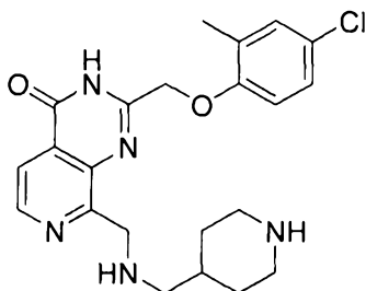
2-((4-chloro-2-methylphenoxy)methyl)-8-(((piperidin-4-ylmethyl)amino)methyl)pyrido[3,4-d]pyrimidin-4(3H)-one
