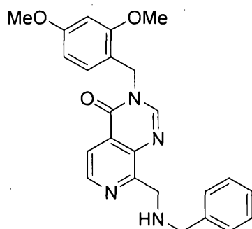
8-((benzylamino)methyl)-3-(2,4-dimethoxybenzyl)pyrido[3,4-d]pyrimidin-4(3H)-one
