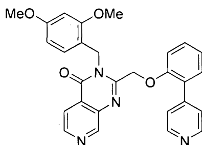
3-(2,4-dimethoxybenzyl)-2-((2-(pyridin-4-yl)phenoxy)methyl)pyrido[3,4-d]pyrimidin-4(3H)-one
