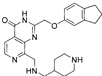
2-(((2,3-dihydro-1H-inden-5-yl)oxy)methyl)-8-(((piperidin-4-ylmethyl)amino)methyl)pyrido[3,4-d]pyrimidin-4(3H)-one
