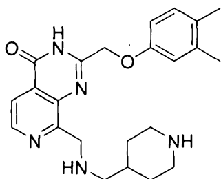
2-((3,4-dimethylphenoxy)methyl)-8-(((piperidin-4-ylmethyl)amino)methyl)pyrido[3,4-d]pyrimidin-4(3H)-one
