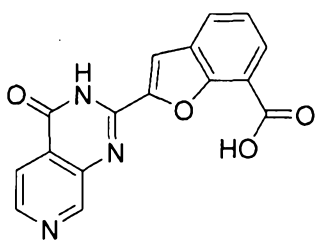
15 2-(4-oxo-3,4-dihydropyrido[3,4-d]pyrimidin-2-yl)benzofuran-7-carboxylic acid
