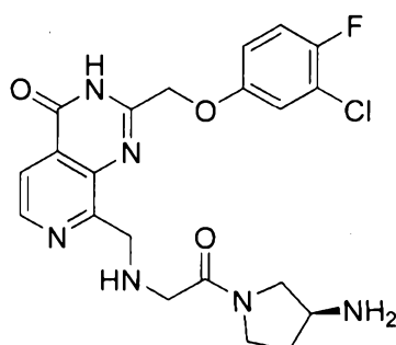
(S)-8-(((2-(3-aminopyrrolidin-1-yl)-2-oxoethyl)amino)methyl)-2-((3-chloro-4-fluorophenoxy)methyl)pyrido[3,4-d]pyrimidin-4(3H)-one
