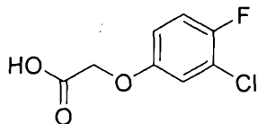
2-(3-chloro-4-fluorophenoxy)acetic acid
