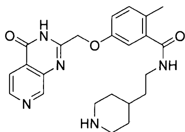
2-methyl-5-((4-oxo-3,4-dihydropyrido[3,4-d]pyrimidin-2-yl)methoxy)-N-(2-(piperidin-4-yl)ethyl)benzamide
