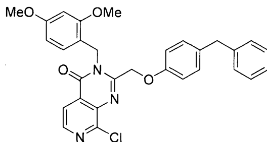
2-((4-benzylphenoxy)methyl)-8-chloro-3-(2,4-dimethoxybenzyl)pyrido[3,4-d]pyrimidin-4(3H)-one
