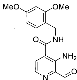
3-amino-N-(2,4-dimethoxybenzyl)-2-formylisonicotinamide
