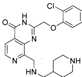
15 2-((2-chlorophenoxy)methyl)-8-(((piperidin-4-ylmethyl)amino)methyl)pyrido[3,4-d]pyrimidin-4(3H)-one
