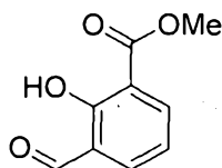
methyl 3-formyl-2-hydroxybenzoate
