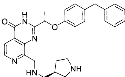
2-(1-(4-benzylphenoxy)ethyl)-8-((((S)-pyrrolidin-3-yl)methyl)amino)methyl)pyrido[3,4-d]pyrimidin-4(3H)-one
