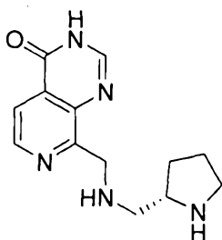
(S)-8-(((pyrrolidin-2-ylmethyl)amino)methyl)pyrido[3,4-d]pyrimidin-4(3H)-one
