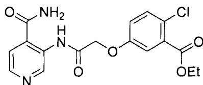
ethyl 5-(2-((4-carbamoylpyridin-3-yl)amino)-2-oxoethoxy)-2-chlorobenzoate
