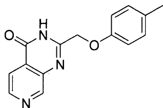
2-((p-tolyloxy)methyl)pyrido[3,4-d]pyrimidin-4(3H)-one
