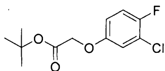
tert-butyl 2-(3-chloro-4-fluorophenoxy)acetate
