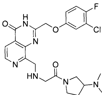
2-((3-chloro-4-fluorophenoxy)methyl)-8-(((2-(3-(dimethylamino)pyrrolidin-1-yl)-2-oxoethyl)amino)methyl)pyrido[3,4-d]pyrimidin-4(3H)-one
