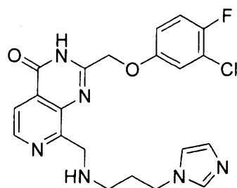
8-(((3-(1H-imidazol-1-yl)propyl)amino)methyl)-2-((3-chloro-4-fluorophenoxy)methyl)pyrido[3,4-d]pyrimidin-4(3H)-one
