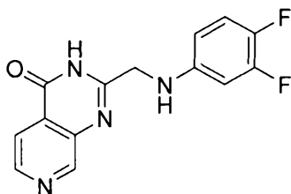
2-(((3,4-difluorophenyl)amino)methyl)pyrido[3,4-d]pyrimidin-4(3H)-one
