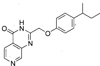
2-((4-(sec-butyl)phenoxy)methyl)pyrido[3,4-d]pyrimidin-4(3H)-one
