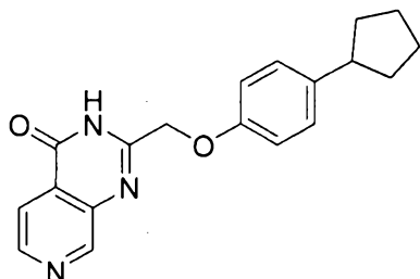
2-((4-cyclopentylphenoxy)methyl)pyrido[3,4-d]pyrimidin-4(3H)-one
