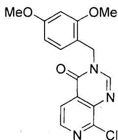
8-chloro-3-(2,4-dimethoxybenzyl)pyrido[3,4-d]pyrimidin-4(3H)-one
