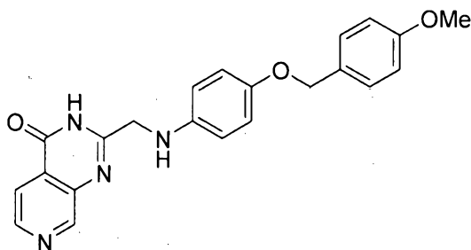
2-(((4-((4-methoxybenzyl)oxy)phenyl)amino)methyl)pyrido[3,4-d]pyrimidin-4(3H)-one
