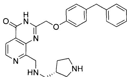
(R)-2-((4-benzylphenoxy)methyl)-8-(((pyrrolidin-3-ylmethyl)amino)methyl)pyrido[3,4-d]pyrimidin-4(3H)-one
