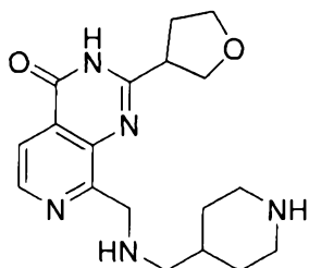
8-(((piperidin-4-ylmethyl)amino)methyl)-2-(tetrahydrofuran-3-yl)pyrido[3,4-d]pyrimidin-4(3H)-one
