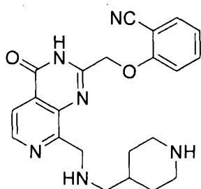
2-((4-oxo-8-(((piperidin-4-ylmethyl)amino)methyl)-3,4-dihydropyrido[3,4-d]pyrimidin-2-yl)methoxy)benzonitrile
