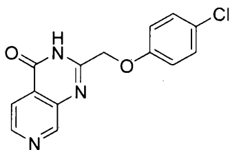
2-((4-chlorophenoxy)methyl)pyrido[3,4-d]pyrimidin-4(3H)-one
