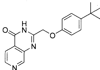
2-((4-(tert-butyl)phenoxy)methyl)pyrido[3,4-d]pyrimidin-4(3H)-one
