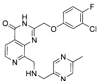
2-((3-chloro-4-fluorophenoxy)methyl)-8-(((5-methylpyrazin-2-yl)methyl)amino)methyl)pyrido[3,4-d]pyrimidin-4(3H)-one
