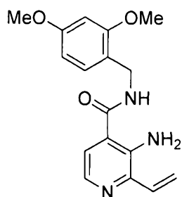
3-amino-N-(2,4-dimethoxybenzyl)-2-vinylisonicotinamide
