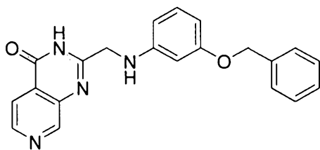
2-(((3-(benzyloxy)phenyl)amino)methyl)pyrido[3,4-d]pyrimidin-4(3H)-one
