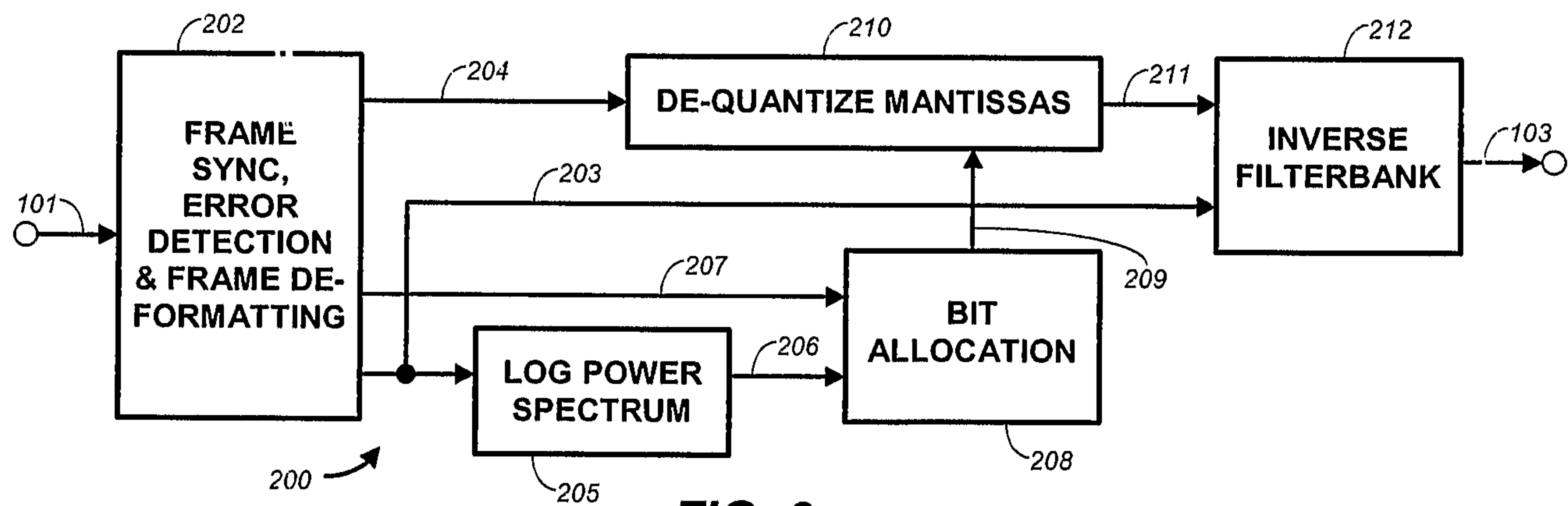
FIG. 2 PRIOR ART
