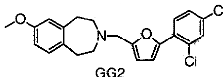
3-[5-(2,4-Dichloro-phenyl)-furan-2-ylmethyl]-7-methoxy-2,3,4,5-tetrahydro-1H-benzo[d]azepine
