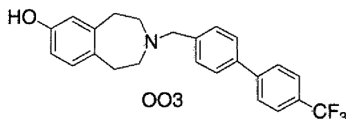
3-(4'-Trifluoromethyl-biphenyl-4-ylmethyl)-2,3,4,5-tetrahydro-1H-benzo[d]azepin-7-ol
