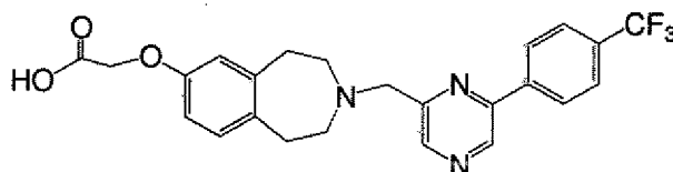
{3-[6-(4-Trifluoromethyl-phenyl)-pyrazin-2-ylmethyl]-2,3,4,5-tetrahydro-1H-benzo[d]azepin-7-yloxy}-acetic acid
