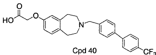
[3-(4'-Trifluoromethyl-biphenyl-4-ylmethyl)-2,3,4,5-tetrahydro-1H-benzo[d]azepin-7-yloxy]-acetic acid
