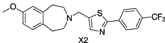
X2 7-Methoxy-3-[2-(4-trifluoromethyl-phenyl)-thiazol-5-ylmethyl]-2,3,4,5-tetrahydro-1H-benzo[d]azepine
