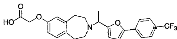
Cpd 28
