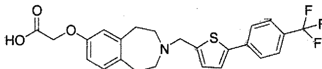
Compound 7
