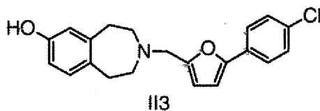
3-[5-(4-Chlorophenyl)-furan-2-ylmethyl]-2,3,4,5-tetrahydro-1H-benzo[d]azepin-7-ol
