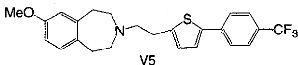
V5 7-Methoxy-3-{2-[5-(4-trifluoromethyl-phenyl)-thiophen-2-yl]-ethyl}-2,3,4,5-tetrahydro-1H-benzo[d]azepine
