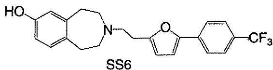
3-{2-[5-(4-Trifluoromethyl-phenyl)-furan-2-yl]-ethyl}-2,3,4,5-tetrahydro-1H-benzo[d]azepin-7-ol
