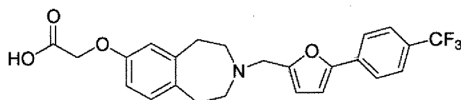
Cpd 9
