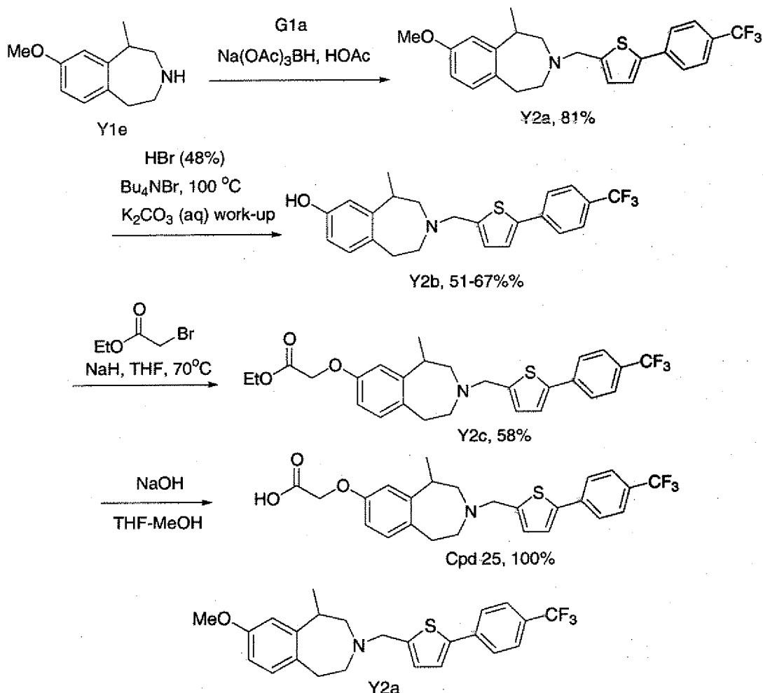
8-Methoxy-1-methyl-3-[5-(4-trifluoromethyl-phenyl)-thiophen-2-ylmethyl]-2,3,4,5-tetrahydro-1H-benzo[d]azepine
