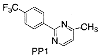
4-Methyl-2-(4-trifluoromethyl-phenyl)-pyrimidine
