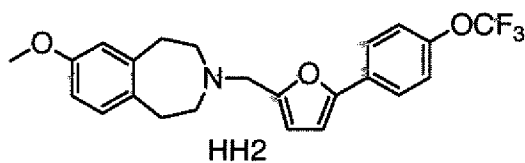
7-Methoxy-3-[5-(4-trifluoromethoxy-phenyl)-furan-2-ylmethyl]-2,3,4,5-tetrahydro-1H-benzo[d]azepine
