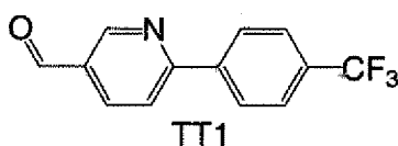
6-(4-Trifluoromethyl-phenyl)-pyridine-3-carbaldehyde
