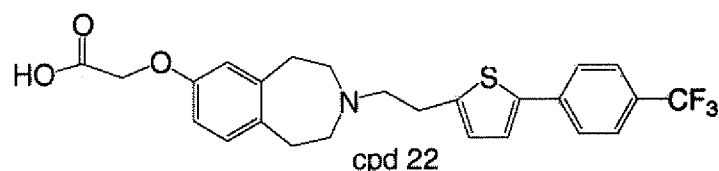
(3-{2-[5-(4-Trifluoromethyl-phenyl)-thiophen-2-yl]-ethyl}-2,3,4,5-tetrahydro-1H-benzo[d]azepin-7-yloxy)-acetic acid
