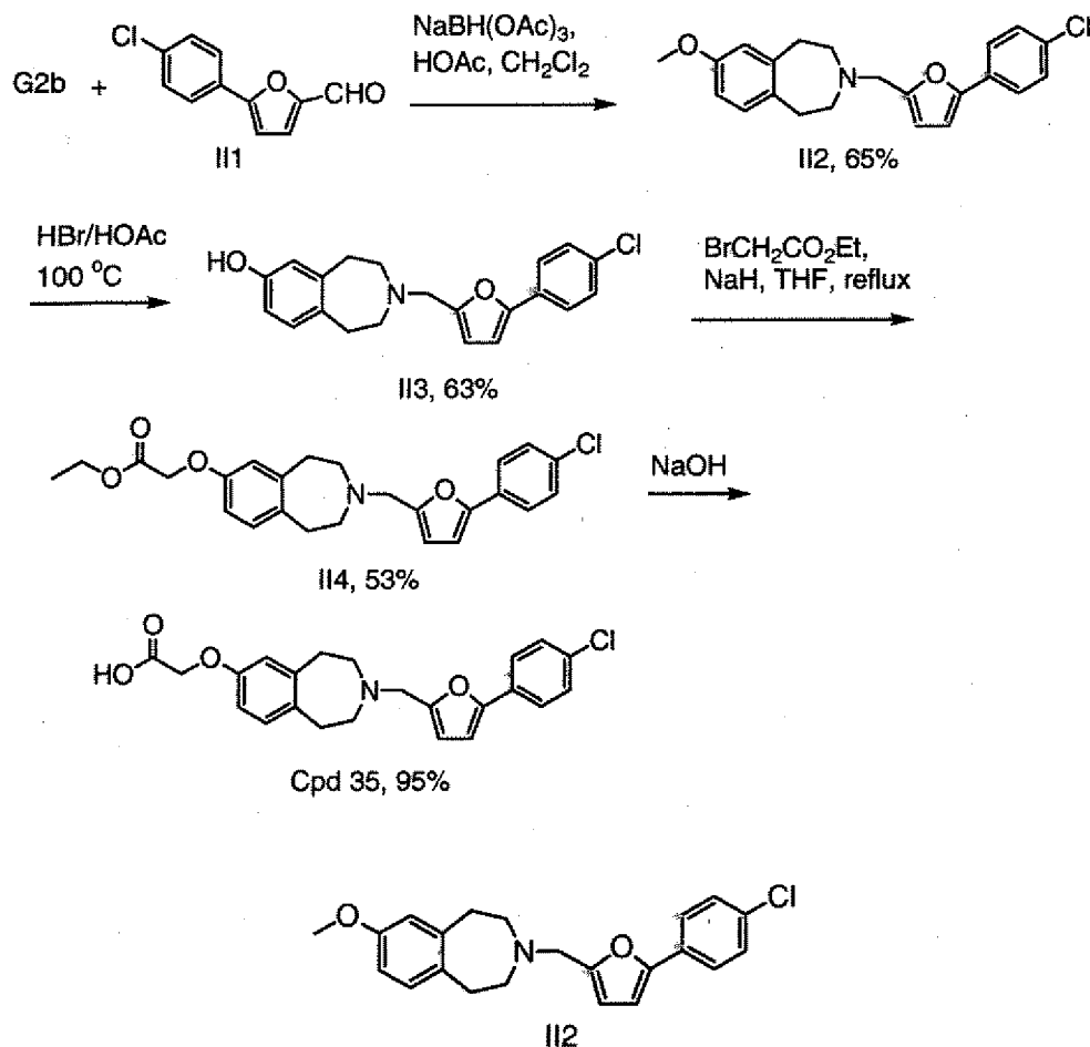
7-Methoxy-3-[5-(4-chlorophenyl)-furan-2-ylmethyl]-2,3,4,5-tetrahydro-1H-benzo[d]azepine
