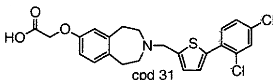
{3-[5-(2,4-Dichloro-phenyl)-thiophen-2-ylmethyl]-2,3,4,5-tetrahydro-1H-benzo[d]azepin-7-yloxy}-acetic acid
