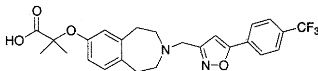
Cpd 12
