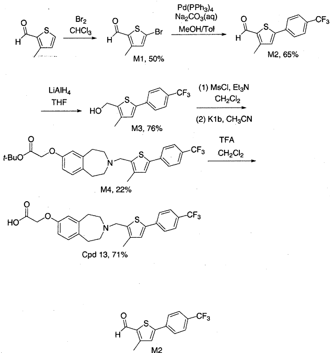
3-Methyl-5-(4-trifluoromethyl-phenyl)-thiophene-2-carbaldehyde
