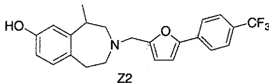
5-Methyl-3-[5-(4-trifluoromethyl-phenyl)-furan-2-ylmethyl]- 2,3,4,5-tetrahydro-1H-benzo[d]azepin-7-ol
