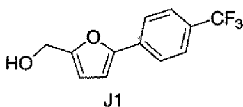
[5-(4-Trifluoromethyl-phenyl)-furan-2-yl]-methanol
