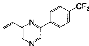
2-(4-Trifluoromethyl-phenyl)-6-vinyl-pyrazine
