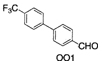
4'-Trifluoromethyl-biphenyl-4-carbaldehyde
