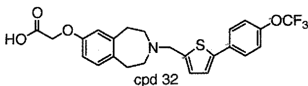
{3-[5-(4-Trifluoromethoxy-phenyl)-thiophen-2-ylmethyl]-2,3,4,5-tetrahydro-1H-benzo[d]azepin-7-yloxy}-acetic acid
