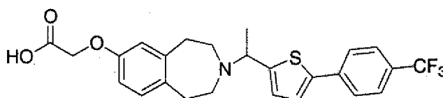
Cpd 27
