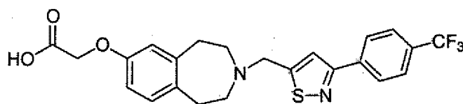
Cpd 1
