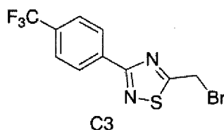
5-Bromomethyl-3-(4-trifluoromethyl-phenyl)-[1,2,4]thiadiazole
