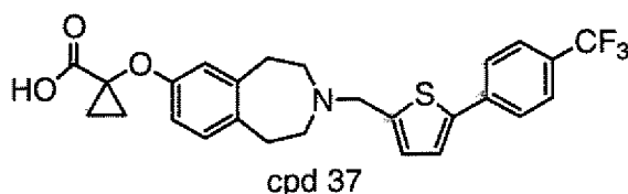
1-{3-[5-(4-Trifluoromethyl-phenyl)-thiophen-2-ylmethyl]-2,3,4,5-tetrahydro-1H-benzo[d]azepin-7-yloxy}-cyclopropanecarboxylic acid
