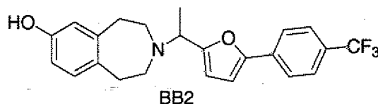
3-{1-[5-(4-Trifluoromethyl-phenyl)-furan-2-yl]-ethyl}-2,3,4,5-tetrahydro-1H-benzo[d]azepin-7-ol
