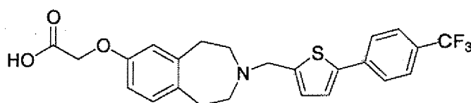
Cpd 7
