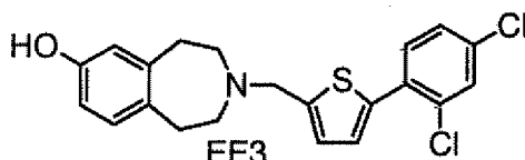
3-[5-(2,4-Dichloro-phenyl)-thiophen-2-ylmethyl]-2,3,4,5-tetrahydro-1H-benzo[d]azepin-7-ol
