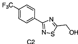
[3-(4-Trifluoromethyl-phenyl)-[1,2,4]thiadiazol-5-yl]-methanol
