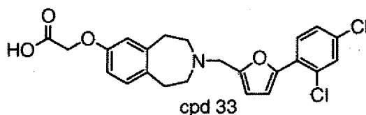
{3-[5-(2,4-Dichloro-phenyl)-furan-2-ylmethyl]-2,3,4,5-tetrahydro-1H-benzo[d]azepin-7-yloxy}-acetic acid
