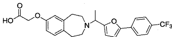
Cpd 28
