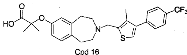
2-Methyl-2-{3-[3-methyl-4-(4-trifluoromethyl-phenyl)-thiophen-2-ylmethyl]-2,3,4,5-tetrahydro-1H-benzo[d]azepin-7-yloxy}-propionic acid
