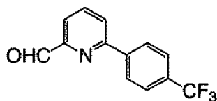
6-(4-Trifluoromethyl-phenyl)-pyridine-2-carbaldehyde
