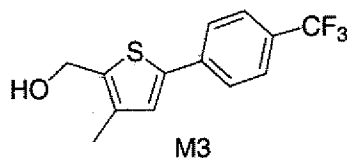
M3 [3-Methyl-5-(4-trifluoromethyl-phenyl)-thiophen-2-yl]-methanol
