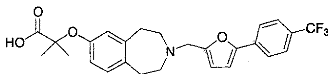
Cpd 10
