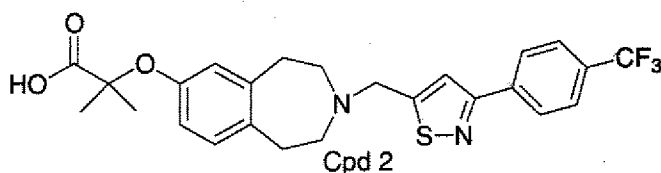
2-Methyl-2-{3-[3-(4-trifluoromethyl-phenyl)-isothiazol-5-ylmethyl]-2,3,4,5-tetrahydro-1H-benzo[d]azepin-7-yloxy}-propionic acid
