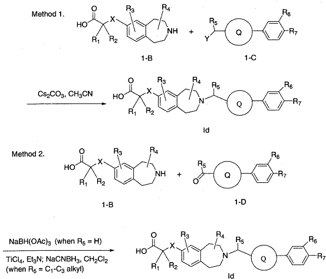
Scheme 1. General methods for the synthesis of Compounds of formula (Id)
