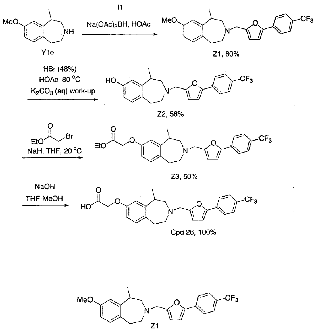
8-Methoxy-1-methyl-3-[5-(4-trifluoromethyl-phenyl)-furan-2-ylmethyl]- 2,3,4,5-tetrahydro-1H-benzo[d]azepine
