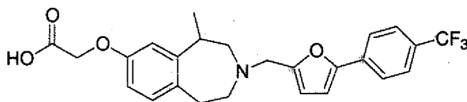
Cpd 26
