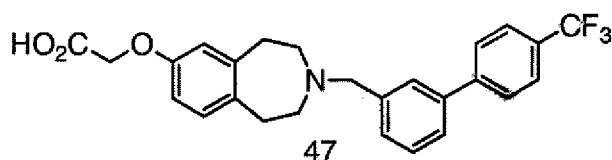
[3-(4'-Trifluoromethyl-biphenyl-3-ylmethyl)-2,3,4,5-tetrahydro-1H-benzo[d]azepin-7-yloxy]-acetic acid
