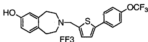
3-[5-(4-Trifluoromethoxy-phenyl)-thiophen-2-ylmethyl]-2,3,4,5-tetrahydro-1H-benzo[d]azepin-7-ol
