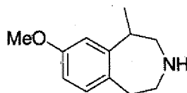
Y1e 8-Methoxy-1-methyl-2,3,4,5-tetrahydro-1H-benzo[d]azepine
