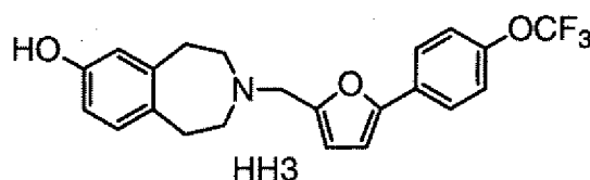
3-[5-(4-Trifluoromethoxy-phenyl)-furan-2-ylmethyl]-2,3,4,5-tetrahydro-1H-benzo[d]azepin-7-ol
