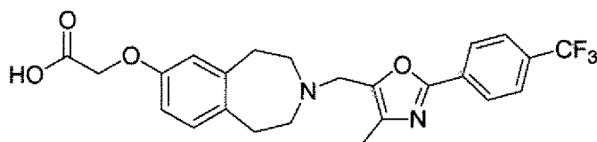
Cpd 18
