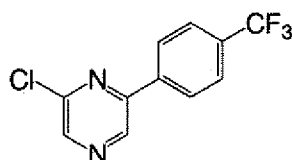
2-Chloro-6-(4-trifluoromethyl-phenyl)-pyrazine
