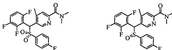
compound A
