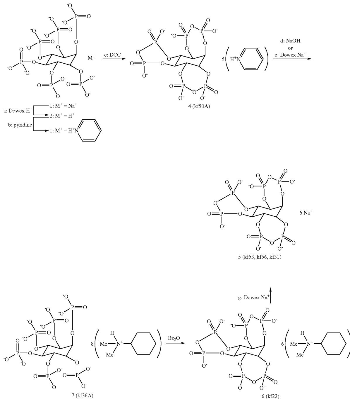
Scheme 3. The ITTP Na salts formation.
