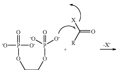
Scheme 2. Mechanism of internal pyrophosphate formation.
