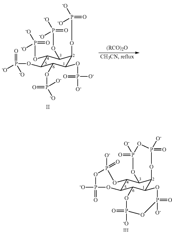
Scheme 1. Synthesis of IHP-tripolyphosphate.
