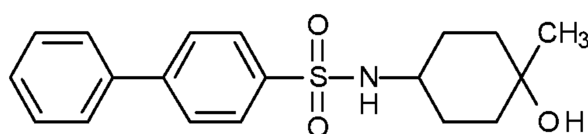
10 N -(4-hydroxy-4-methyl-cyclohexyl)-4-phenyl-benzenesulfonamide
