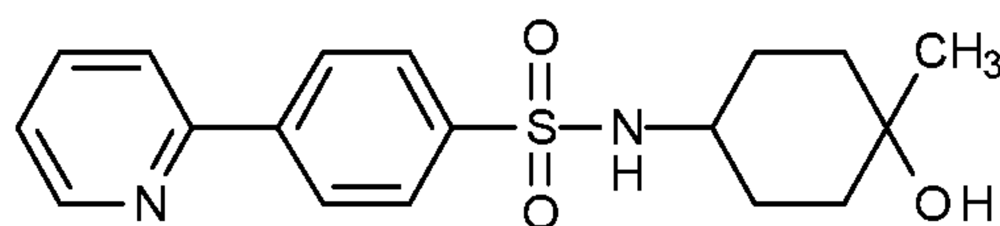
15 N -(4-hydroxy-4-methyl-cyclohexyl)-4-(2-pyridyl)benzenesulfonamide
