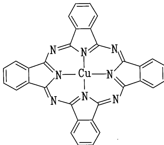
Copper(II) phthalocyanine (CuPc)
