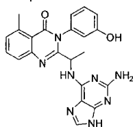
2-[1-(2-Amino-9H-purin-6-ylamino)-ethyl]-3-(3-hydroxy-phenyl)-5-methyl-3H-quinazolin-4-one (132)
