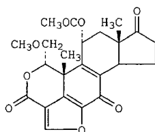
wortmannin
