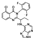
(174)
