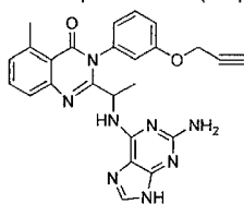
2-[1-(2-Amino-9H-purin-6-ylamino)-ethyl]-5-methyl-3-(3-prop-2-ynyloxy-phenyl)-3H-quinazolin-4-one (136)
