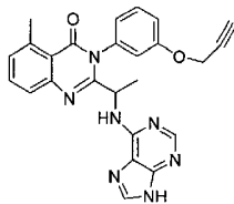
5-Methyl-3-(3-prop-2-ynyloxy-phenyl)-2-[1-(9H-purin-6-ylamino)-ethyl]-3H-quinazolin-4-one (131)
