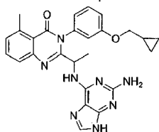
2-[1-(2-Amino-9H-purin-6-ylamino)-ethyl]-3-(3-cyclopropylmethoxy-phenyl)-5-methyl-3H-quinazolin-4-one (135)
