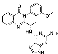
2-[1-(2-Amino-9H-purin-6-ylamino)-ethyl]-3-(3-methoxy-phenyl)-5-methyl-3H-quinazolin-4-one (134)
