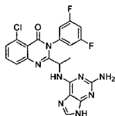
(172)
