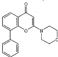
LY294002
