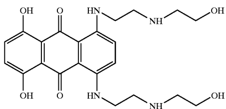
Mitoxantrone
