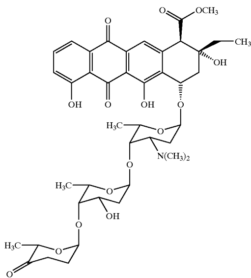
Aclacinomycin A
